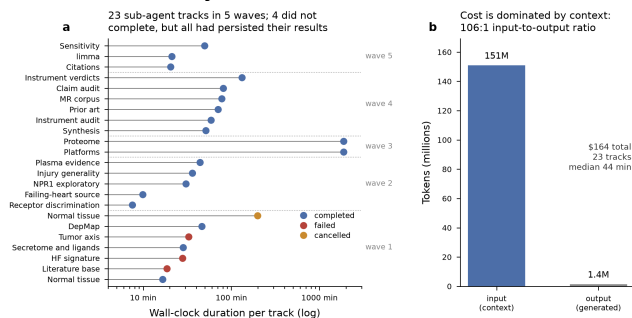
Figure 1. The multi-agent system that executed the analysis. (a) Wall-clock duration of each of the 23 sub-agent tracks, grouped into the five dispatch waves and colored by terminal status. The two longest tracks (Proteome, Platforms) include time parked on user approvals for network access. All four non-completing tracks had already written their results to the artifact store, and every one of those artifacts is cited in this paper. (b) Token consumption across the fleet. Cost is context rather than generation, which is why re-running the analysis from the six skills requires no model at all. Per-track figures are given in delegation_record.csv .
