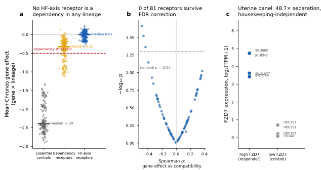
Figure 5. Receptor expression and CRISPR dependency. (a) HF-axis receptors cluster at zero gene effect while essential controls sit near -2.4 . (b) No receptor survives FDR. (c) Proposed uterine panel.
