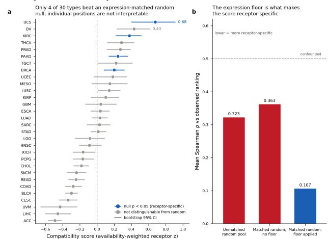
Figure 4. Pan-cancer compatibility ranking against an expression-matched null. (a) Ranking with bootstrap CIs; the 4 blue types beat the matched-random null at p < 0.05 . (b) The floor is what makes the score receptor-specific.
