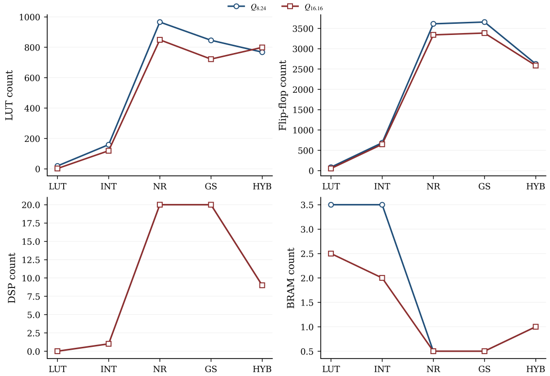
Fig. 23. Full resource utilization (LUT, FF, DSP, BRAM) by architecture, Q8.24 vs. Q16.16.
