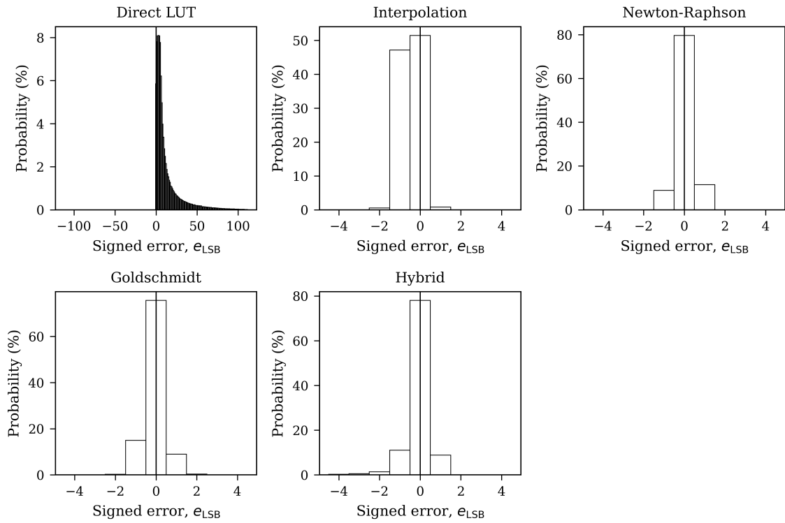
Fig. 14. Signed error distributions by architecture, Q16.16 (raw LSB units).
