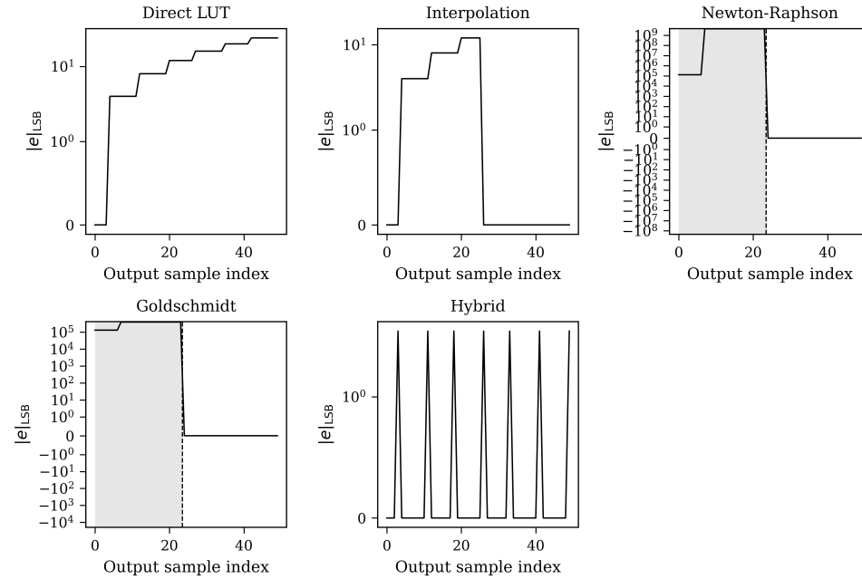
Fig. 18. Pipeline warm-up transient by architecture (shaded region = pipeline fill period), Q16.16.
