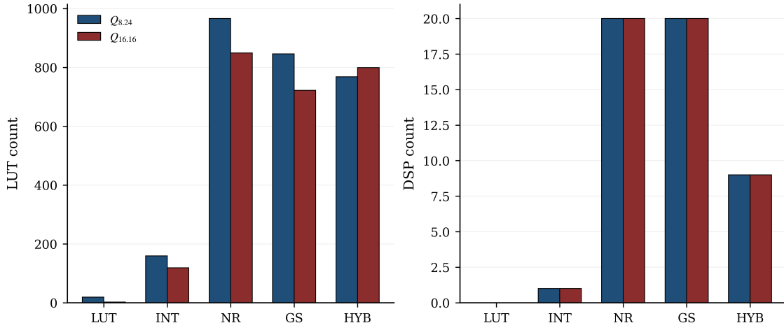
Fig. 21. LUT and DSP utilization by architecture, Q8.24 vs. Q16.16.
