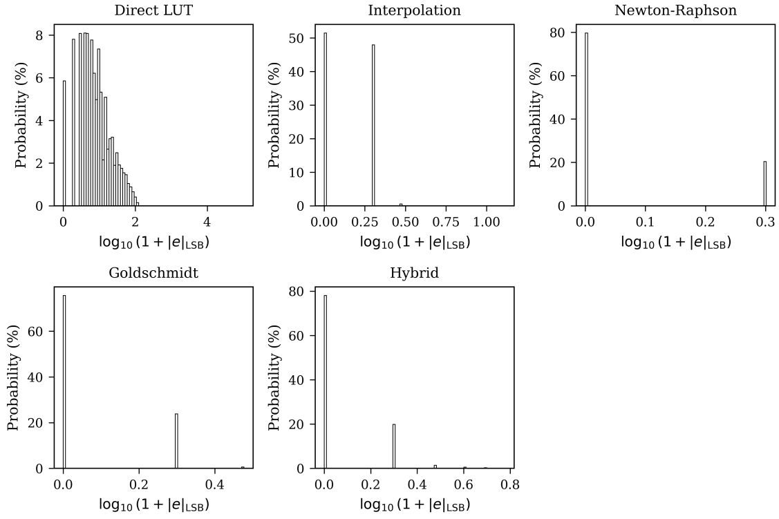
Fig. 15. Absolute error distributions by architecture, Q16.16 ( \log_{10}(1 + |e|) scale).
