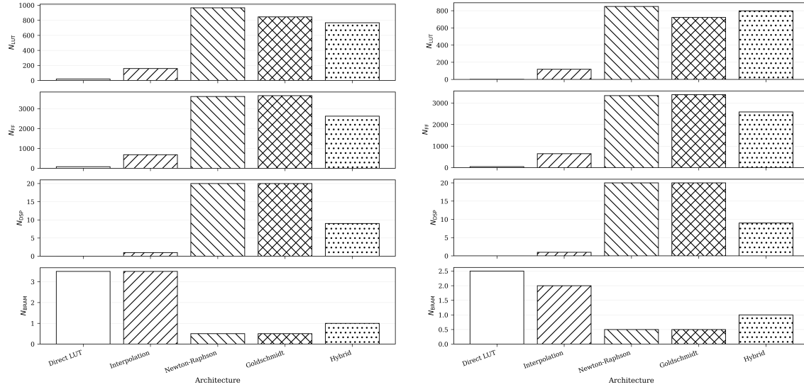
Fig. 6. Post-implementation LUT, flip-flop, DSP, and BRAM utilization by architecture, Q8.24(left) &amp; Q16.16(right)
