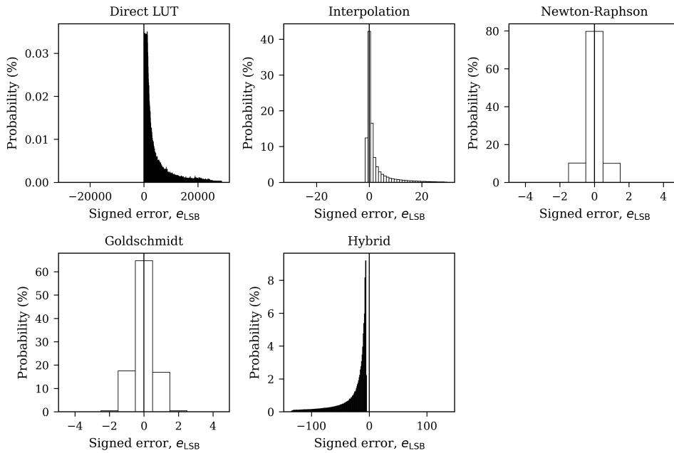
Fig. 8. Signed error distributions by architecture, Q8.24 (raw LSB units).
