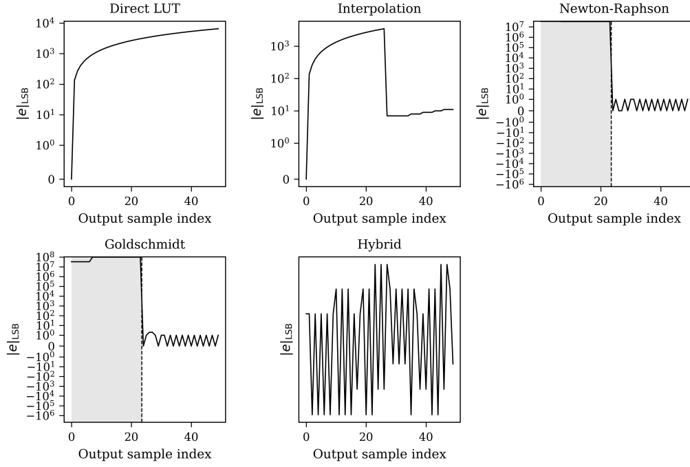
Fig. 12. Pipeline warm-up transient by architecture (shaded region = pipeline fill period), Q8.24.
