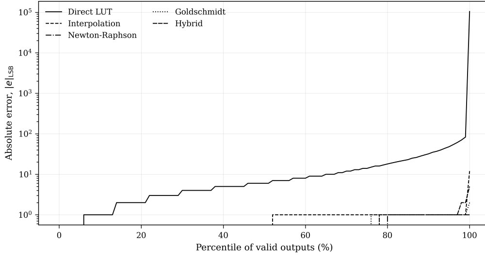
Fig. 19. Absolute error as a function of output percentile, all architectures, Q16.16.
