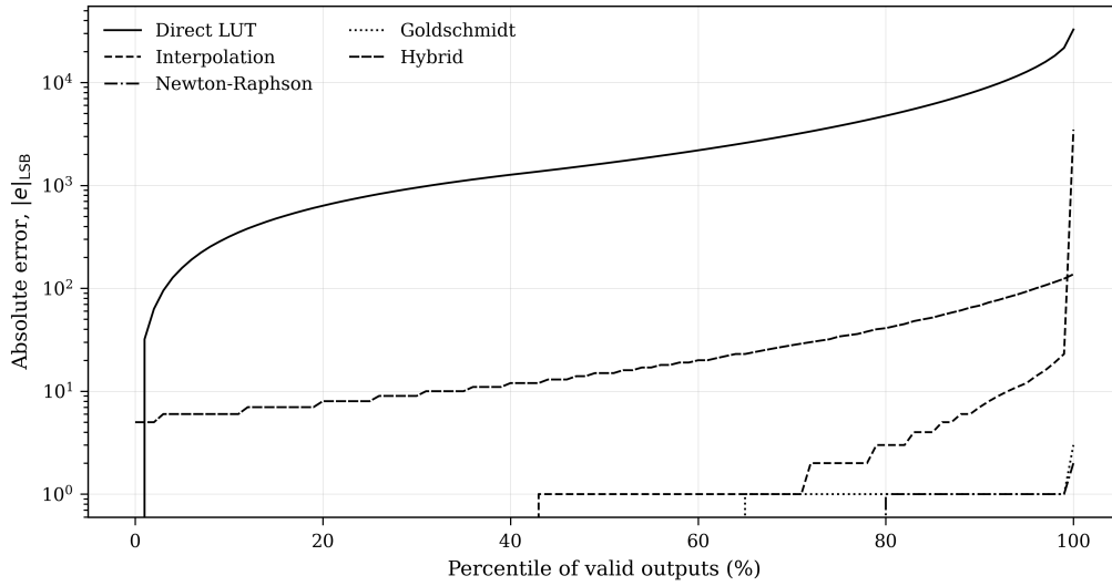
Fig. 13. Absolute error as a function of output percentile, all architectures, Q8.24.
