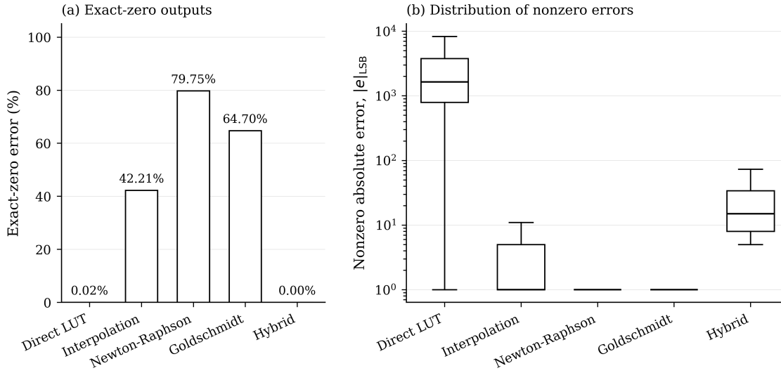
Fig. 10. Zero-LSB output fraction and distribution of nonzero errors by architecture, Q8.24.
