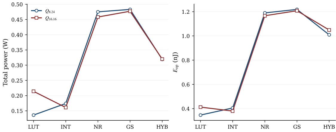
Fig. 22. Total power and energy per operation by architecture, Q8.24 vs. Q16.16.
