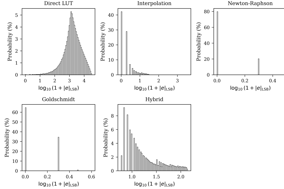
Fig. 9. Absolute error distributions by architecture, Q8.24 ( \log_{10}(1 + |e|) scale).
