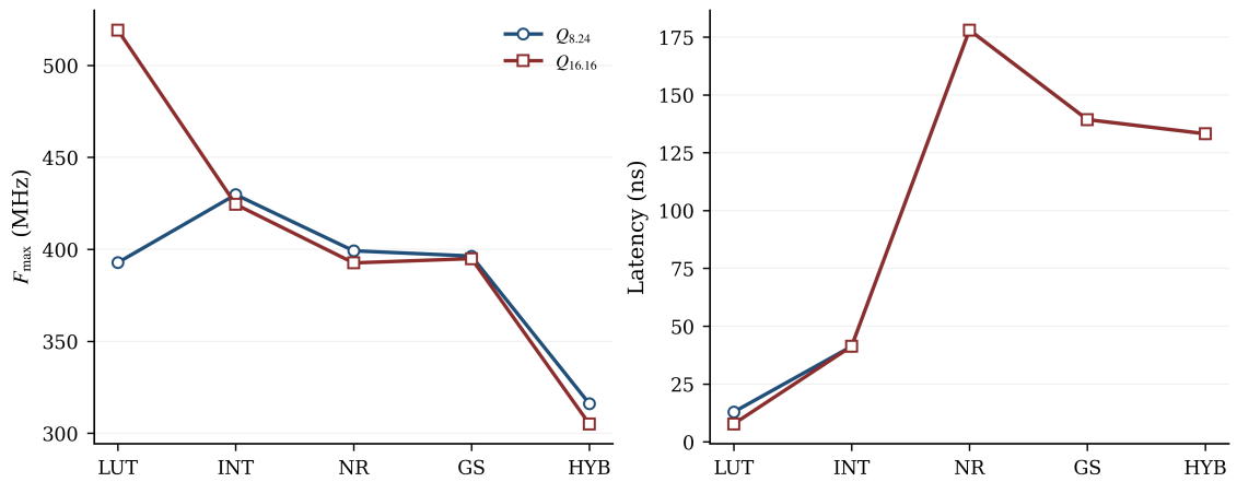
Fig. 20. Achieved F_{\max} and latency (ns) by architecture, Q8.24 vs. Q16.16.
