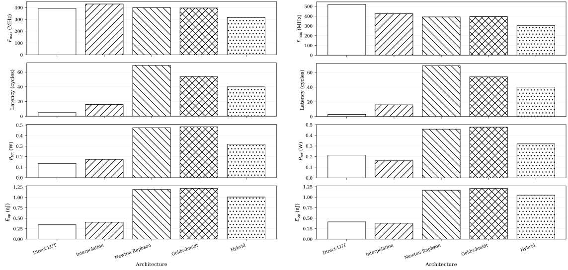
Fig. 7. Post-implementation F_{\max} , latency (cycles), total power, and energy per operation by architecture, Q8.24(left) & Q16.16(right)
