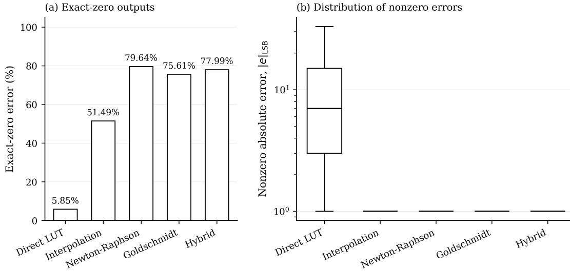
Fig. 16. Zero-LSB output fraction and distribution of nonzero errors by architecture, Q16.16.
