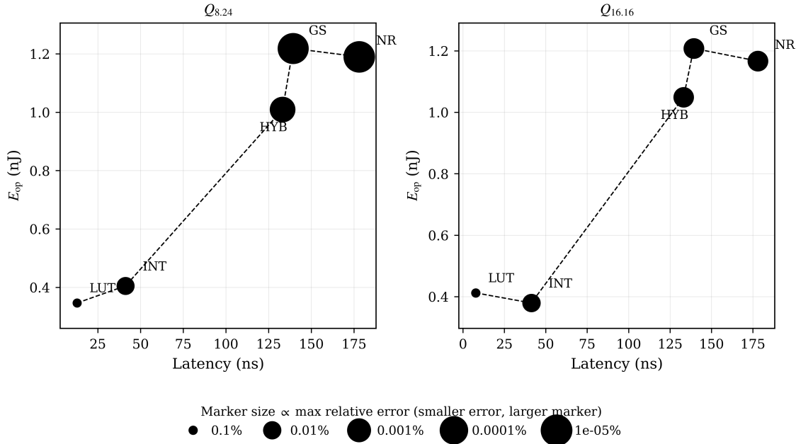
Fig. 26. Pareto trade-off in the latency-energy plane, by architecture, Q8.24 (left) and Q16.16 (right). Marker size is proportional to accuracy (max relative error) on a shared global scale across both panels; all five architectures are mutually non-dominated in both formats.
