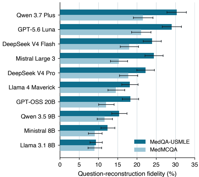
A How often the hidden question can be reconstructed
