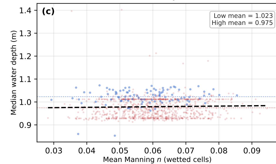
HEC-RAS — median depth (CV=4.6%)
