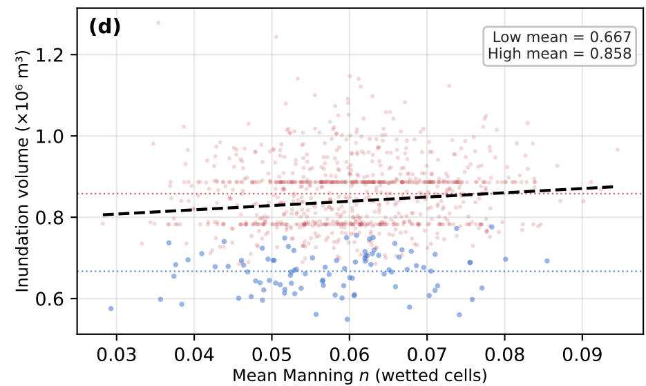
HEC-RAS — inundation volume (CV=11.7%)
