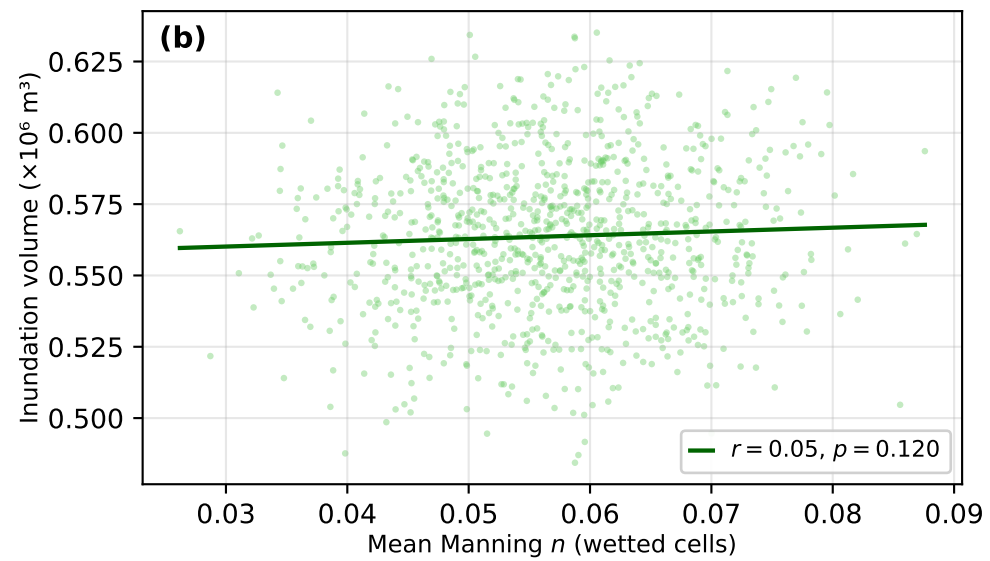
SFINCS — inundation volume (CV=4.8%)
