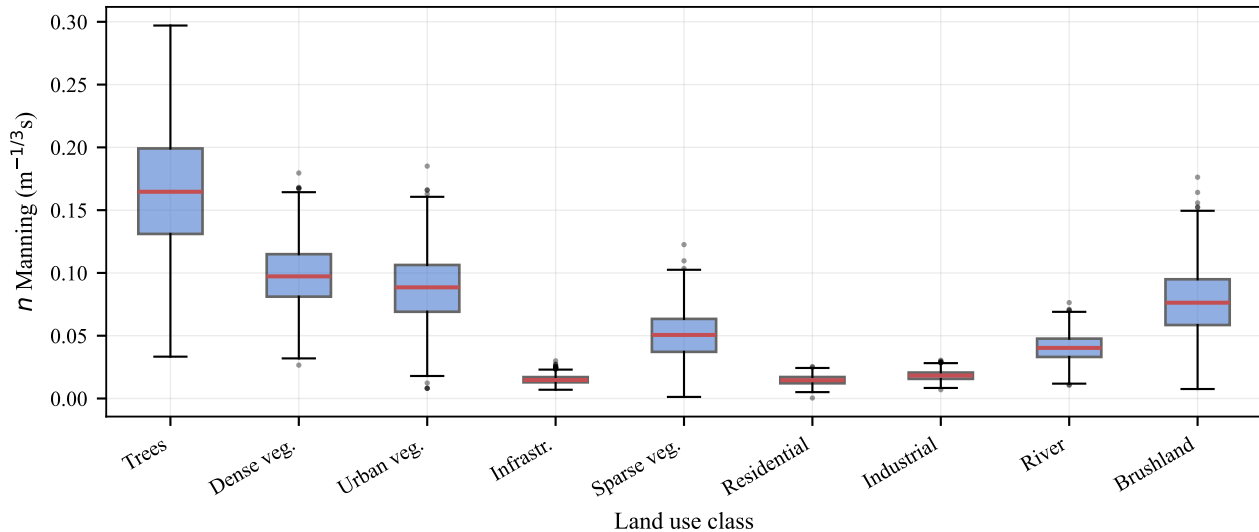
Monte Carlo ensemble: 1,000 Manning combinations — 9 land use classes
