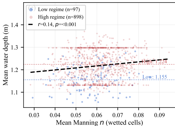
HEC-RAS — CV=5.7% (bimodal: two bands)
