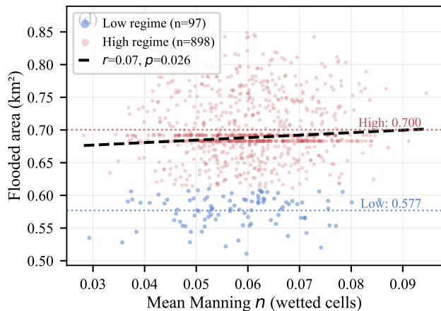
HEC-RAS — CV=8.4% (bimodal: two bands)
