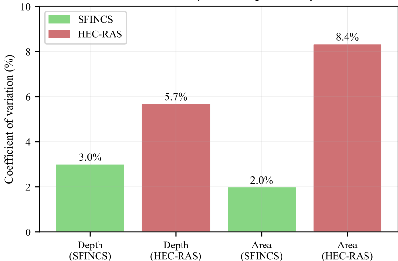
Model sensitivity to Manning uncertainty
