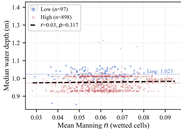
HEC-RAS — depth_median (CV=4.6%)
