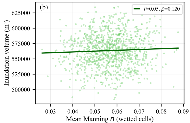
SFINCS — volume_m3 (CV=4.8%)
