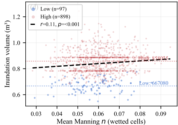
HEC-RAS — volume_m3 (CV=11.7%)
