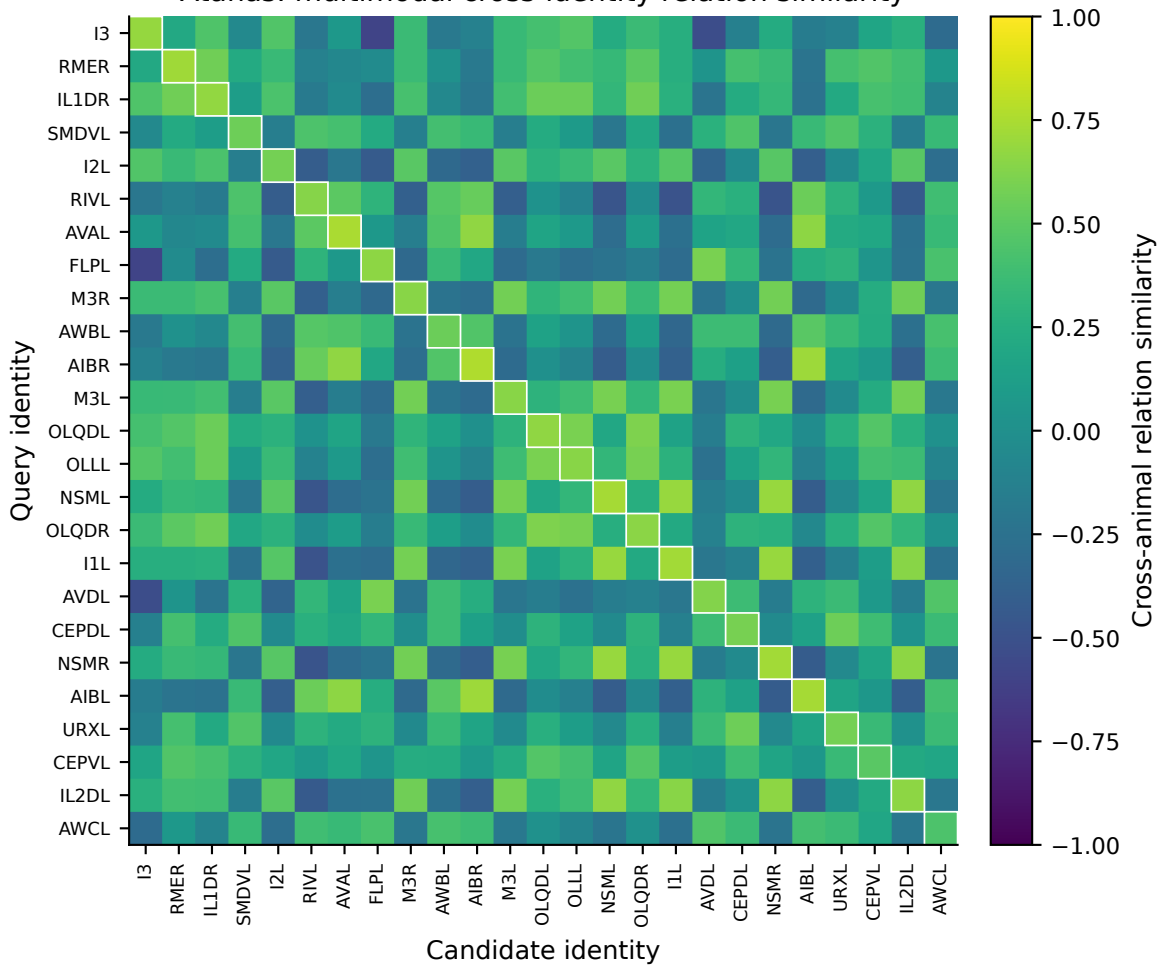
Atanas: multimodal cross-identity relation similarity
