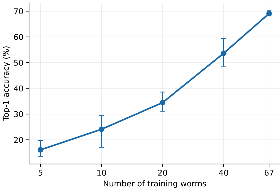
RLD training-population scaling (val)
