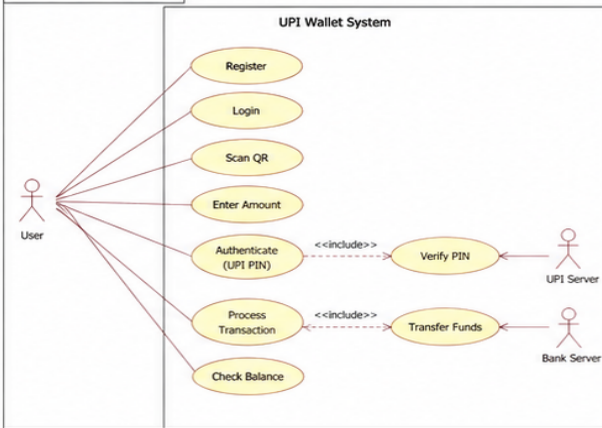
1. USE CASE DIAGRAM
