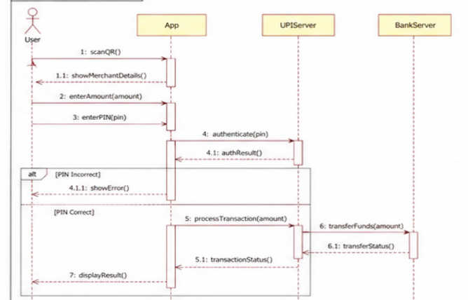
3. SEQUENCE DIAGRAM
