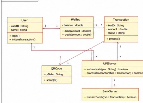
2. CLASS DIAGRAM
