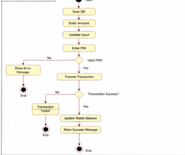
5. ACTIVITY DIAGRAM
