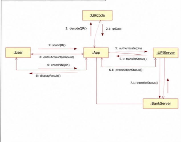
4. COLLABORATION (COMMUNICATION) DIAGRAM
