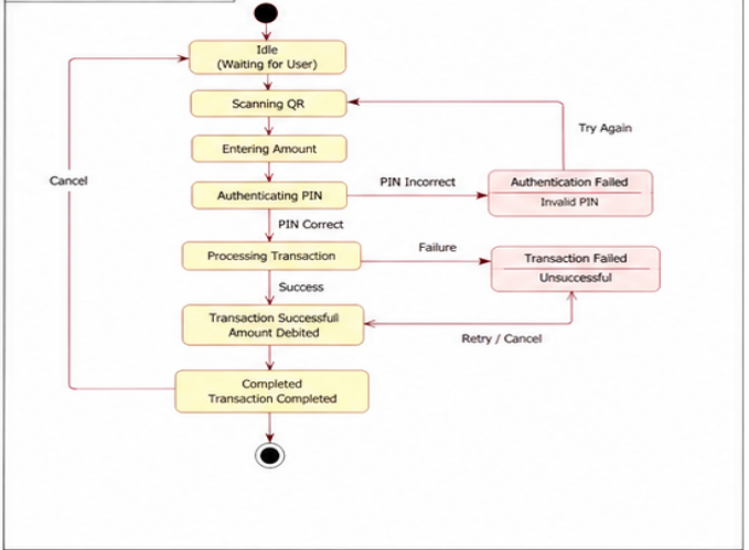
6. STATE CHART DIAGRAM
