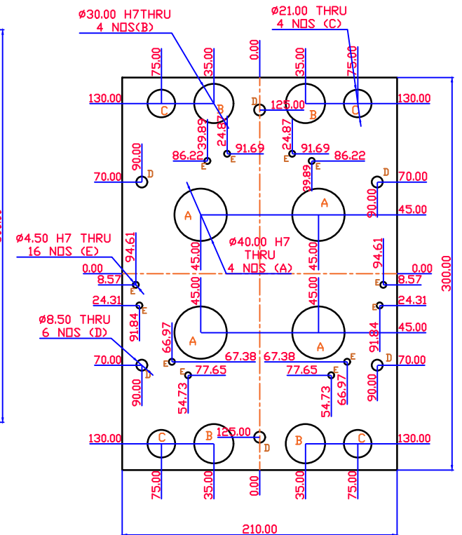
Top view EJECTOR PLATE
