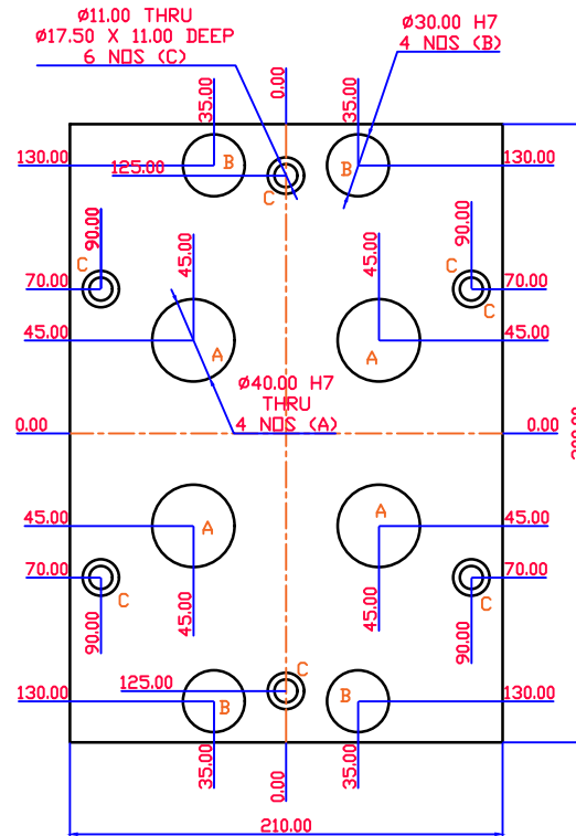
Top view EJECTOR BACK PLATE
