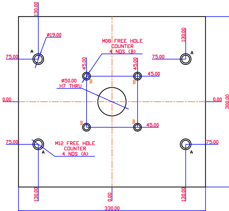
Top view BOTTOM PLATE
