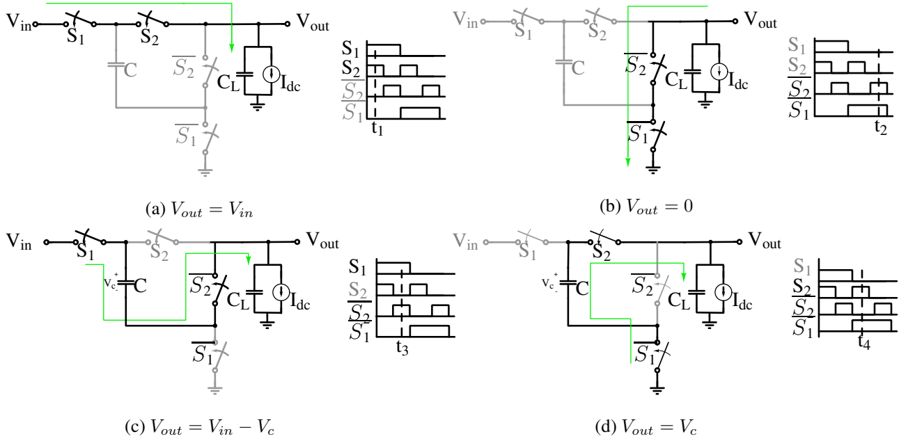
Figure 4.6: Different output levels that can be generated by 3-level flying capacitor multi-level converter and the corresponding control signals for complementary switches.
