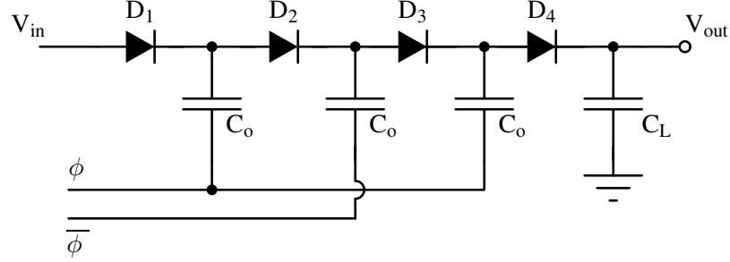
Figure 2.9: Schematic of conventional Dickson charge pump.
