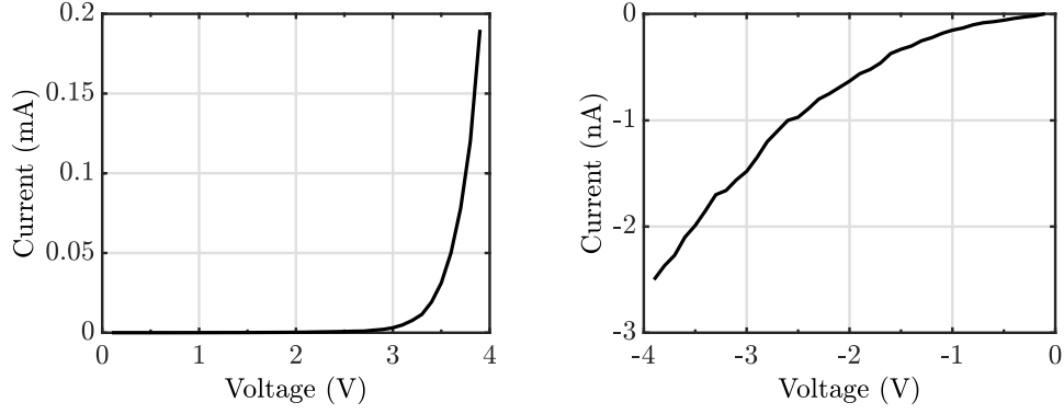
(c) Forward and reverse characteristics of diode-3 between pins 6 & 7.
