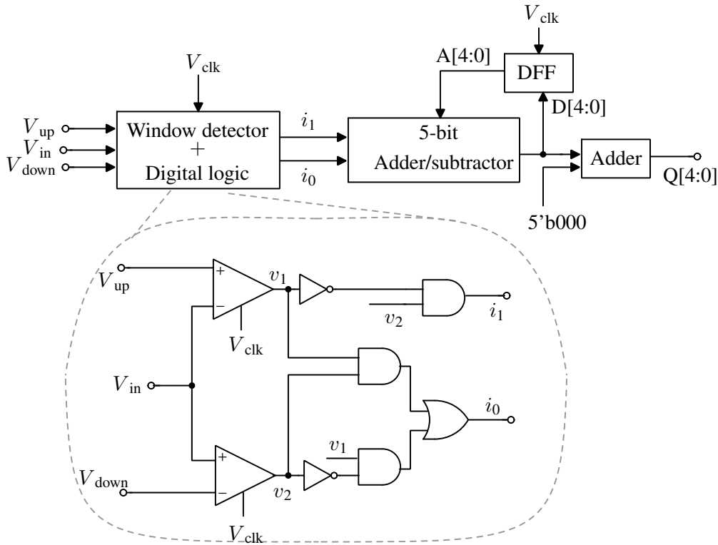
Figure 3.18: Block diagram of digital control logic. V_{up} and V_{down} are the pre-defined threshold against which the input is compared. The 5-bit digital word, Q generated by this block controls the efficiency of the charge pump by varying the number of capacitors that should be coupled with the clock signal.
