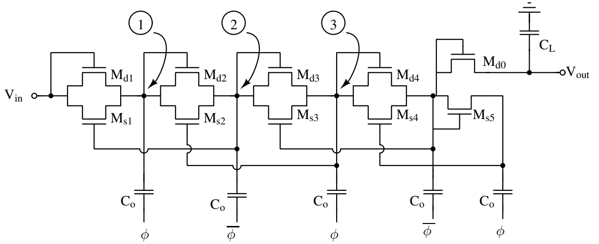
Figure 2.14: Schematic of a 4-stage static CTS based Dickson charge pump. M_{sk} are auxiliary switches with static backward control that direct the flow of charge during pumping operation.
