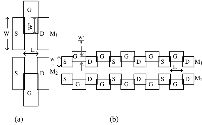
Figure 2.3: (a) Differentially arranged SGFET, (b) shows the fingered version of the same. The sensitivity of the SGFET gets multiplied by the number of fingers n , as any displacement affects all the fingers equally.
