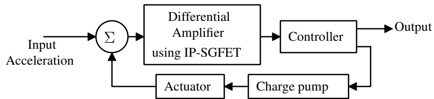
Figure 3.1: Block diagram of closed-loop accelerometer system [44,45].
