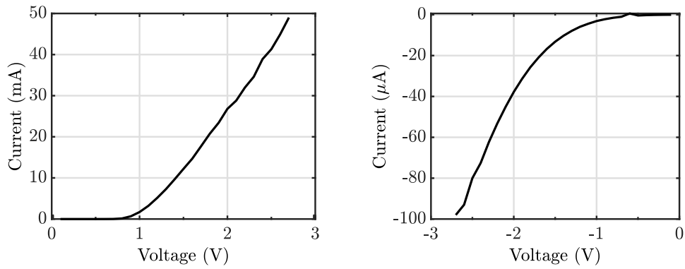
(e) Forward and reverse characteristics of diode-5 between pins 15 & 16.
