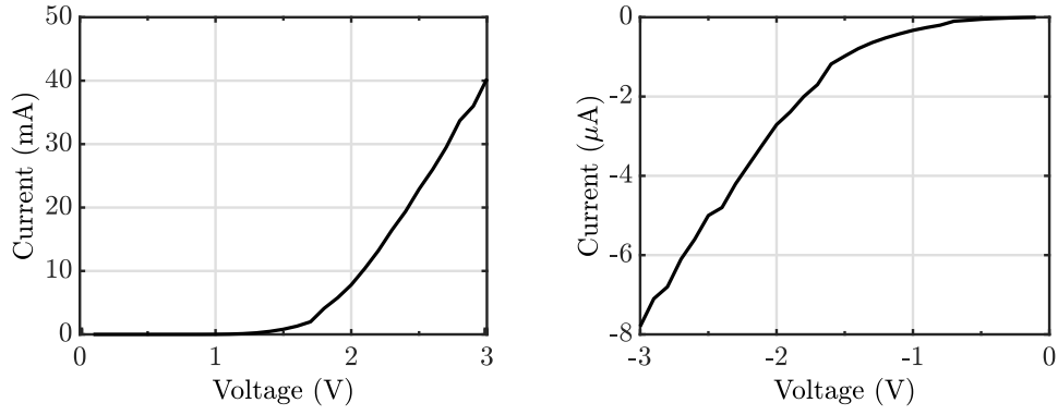
(d) Forward and reverse characteristics of diode-4 between pins 13 & 14.
