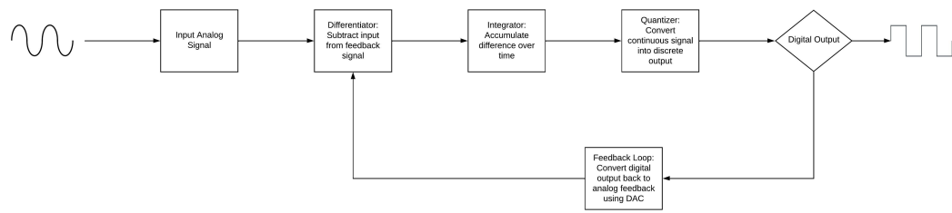
Figure 2.4: Sigma-Delta ( \Sigma - \Delta ) modulator
