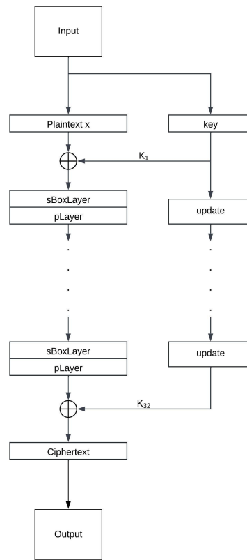
Figure 3.4: PRESENT Algorithm.[3][4]
