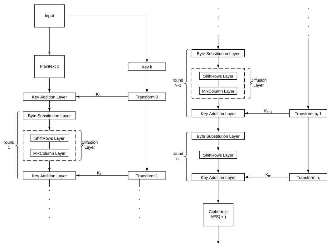
Figure 3.5: AES Algorithm.[3]
