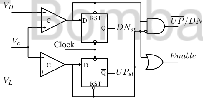
Figure 4.9: Control logic for generating \overline{UP}/DN and Enable signals for the ring counter and UP_{st} & DN_{st} signals for the strong charge pump. V_H , V_L are the upper and lower thresholds of window comparator respectively.
