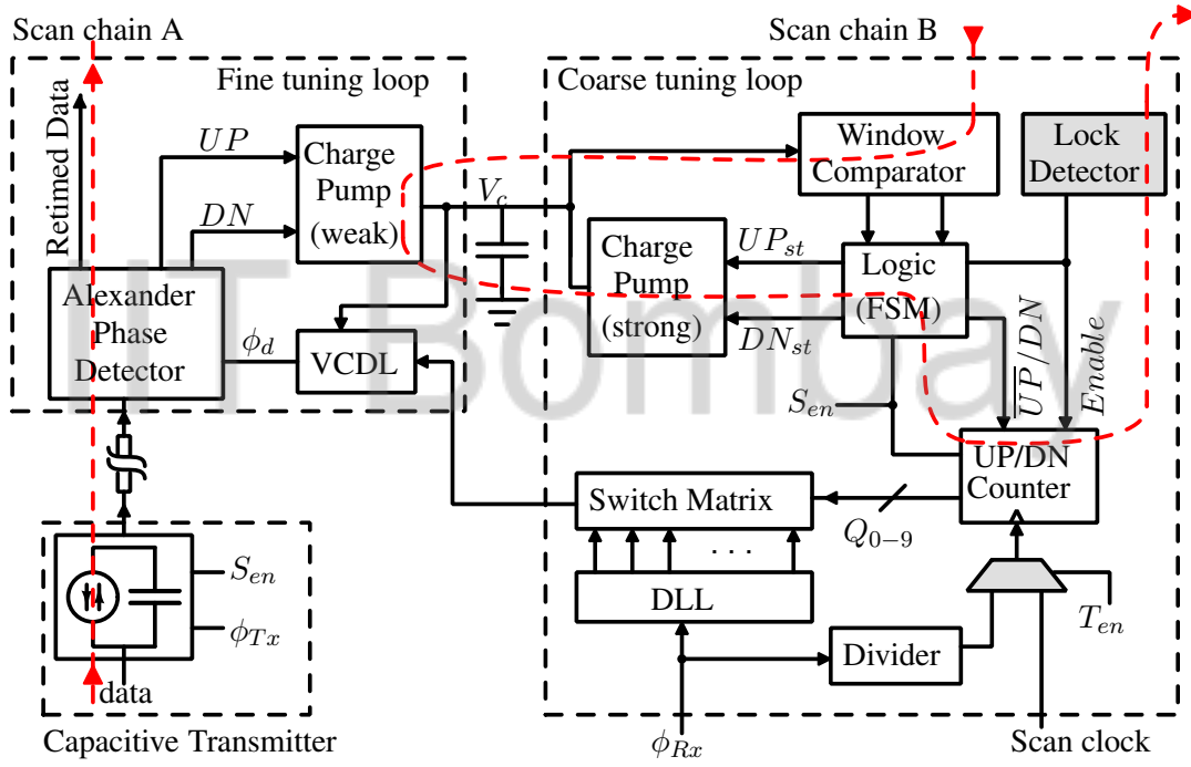
Figure 5.2: Block diagram clock synchronizer system, divided into fine tuning and coarse tuning loops. S_{en} : Scan enable signal, T_{en} : Test mode enable.
