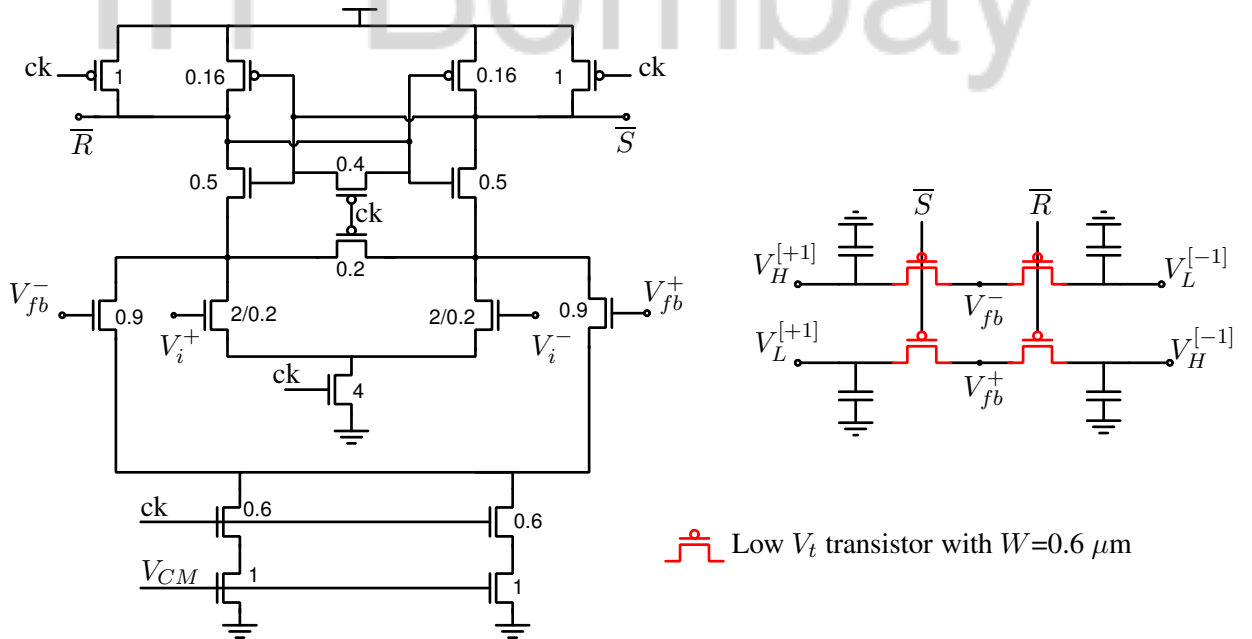
Figure 3.29: DFE circuit implemented in UMC 130 nm technology, with transistor dimensions. All dimensions are in \mu\text{m} . Unless explicitly mentioned, length of all transistors is minimum which is 120 nm.
