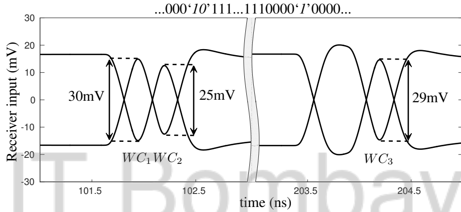
Figure 3.9: Receiver input voltage : \lambda_2 is more than optimum.
