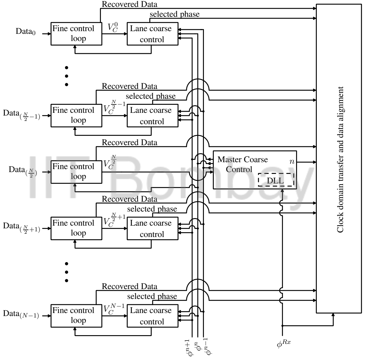
Figure 7.1: A suggested architecture for a mesochronous clock retiming circuit for a bus interconnect.
