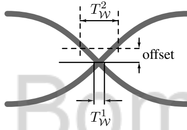
Figure 6.3: Illustration of the sampler offset increasing the size of the window \mathcal{W} from T_{\mathcal{W}}^1 to T_{\mathcal{W}}^2 .
