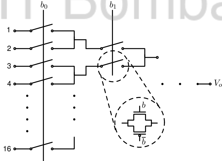
Figure 3.28: The circuit diagram of the switch matrix used in the DAC in Figure 3.27. Four such switch matrices are used to tap the resistor ladder to generate the required four bias voltages.
