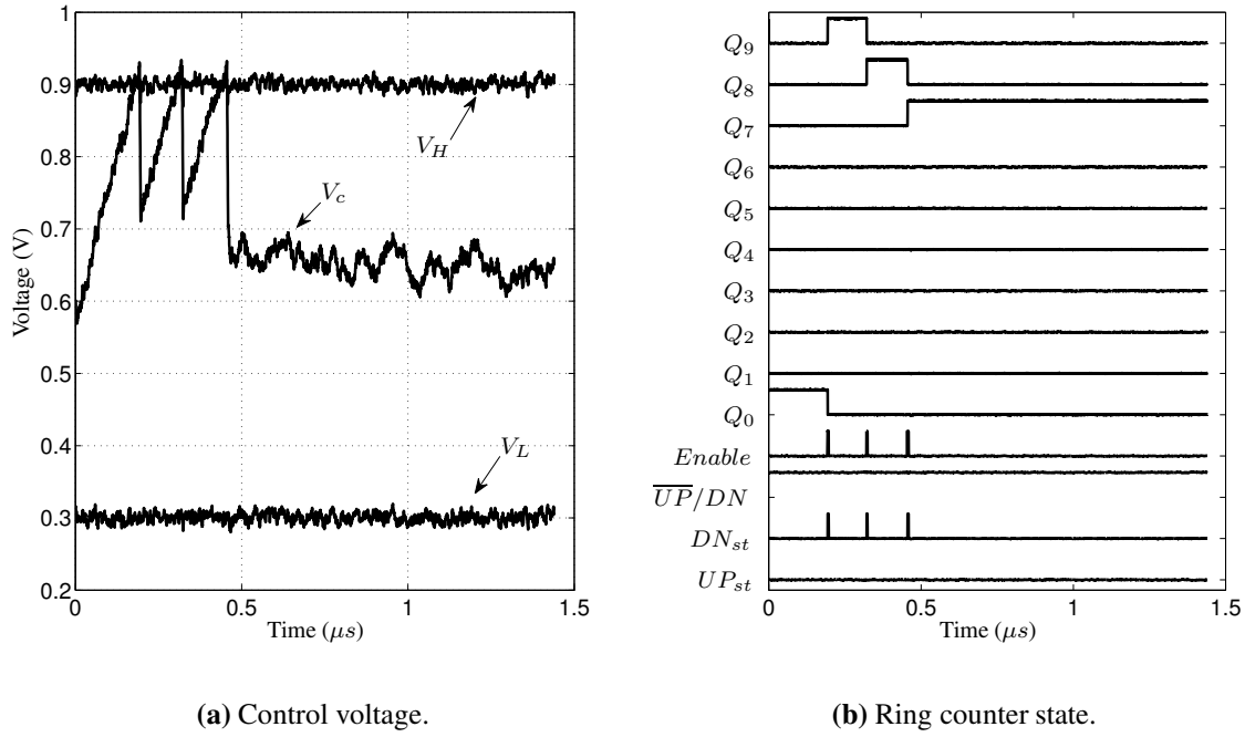
Figure 4.7: Control signals of the continuous phase clock synchronizer obtained from layout extracted simulations. 5% noise was added to the supply for this simulation.
