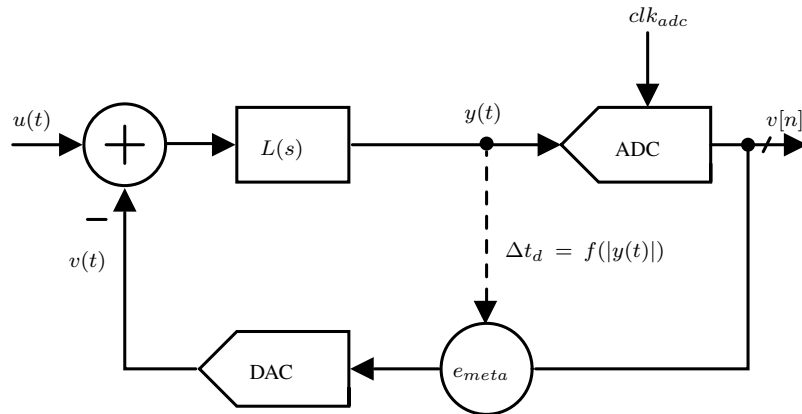
Figure 3.31: Metastability induced error model in CTDSM [21].
