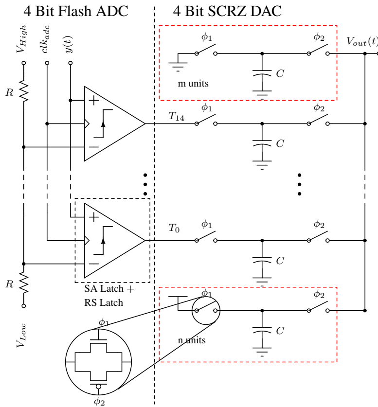
Figure 4.11: Cascade of 4 Bit Flash ADC with 4 Bit DAC based on switched-capacitor resistors used in CTDSM. The input dynamic range of ADC is controlled by V_{High} and V_{Low} , whereas DAC's output dynamic range is controlled by adjusting the number of always ON and OFF (m,n) unit elements.
