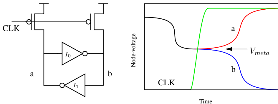
Figure 2.11: Perfectly matched Cross-coupled inverter pair pre-charged to VDD enters metastability. Random noise at nodes a and b introduces variability during each clock evaluation phase, resulting in a random resolution state.
