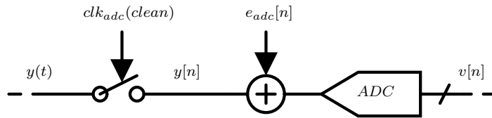
Figure 3.24: e_{adc}[n] is error induced due to jitter in clk_{adc} , which is modeled to be added at the input of the ADC within CTDSM.
