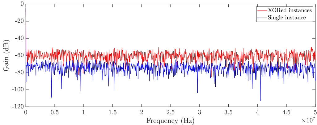
Figure 4.7: Spectrum of a single instance of 4 Bit CTDSM LSB output (blue) along with its four XORed instances (red).
