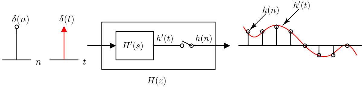
Figure 3.7: Impulse-invariant transformation
