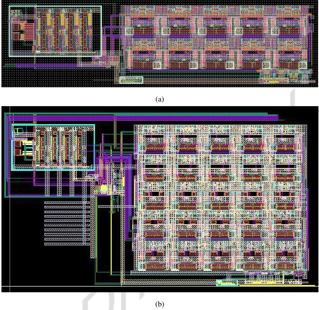
Figure 4.16: Layout of (a) 10-stage (b) 25-stage expansion circuits with PULSEGEN and other blocks.
