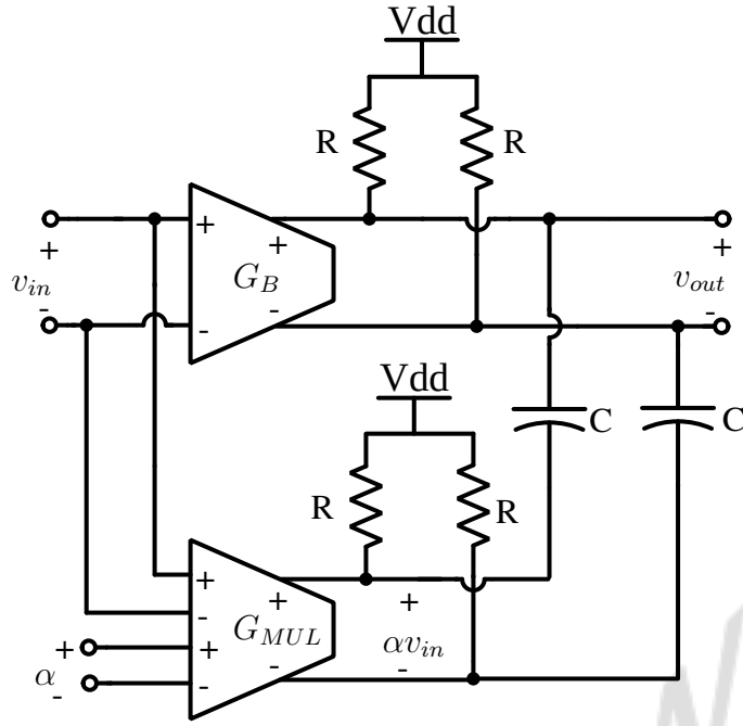
Figure 3.5: Block level representation of variable delay circuit using transconductors: G_B and G_{MUL} .
