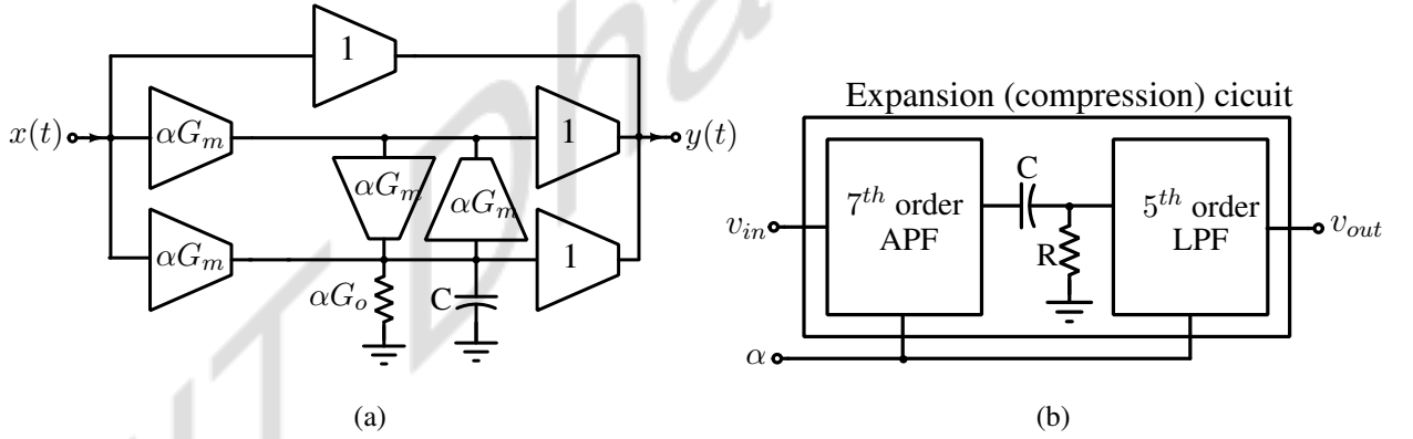
Figure 2.13: (a) G_m -C implementation of second order filter with multiplier \alpha , (b) Block diagram of expansion (compression) circuit.
