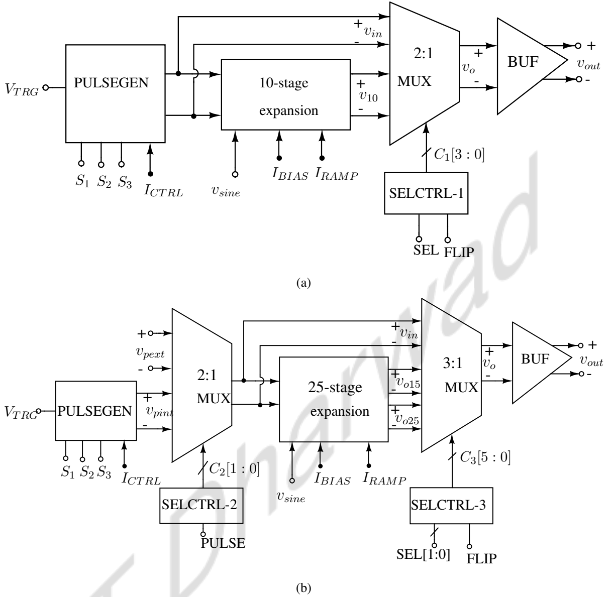
Figure 4.10: Simplified architecture of test setup for testing (a) 10-stage and (b) 25-stage pulse expansion circuits.
