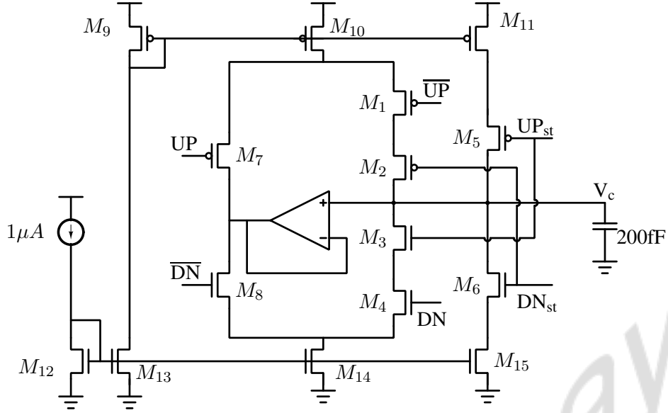
Figure 4.22: The weak and the strong charge pump. DN, \overline{\text{DN}} , UP and \overline{\text{UP}} are from the fine tuning loop and \text{UP}_{\text{st}} and \text{DN}_{\text{st}} are from the coarse tuning loop.
