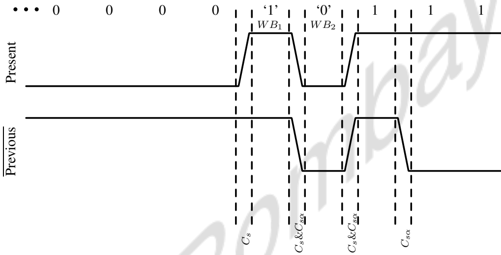
Figure 3.4: The worst case sequence WC_1 (which is same as WC_2 except for the bit under examination), used to design the two tap equalizer. The upper signal is the data signal and the lower signal is a 1-bit delayed and inverted version of the same.
