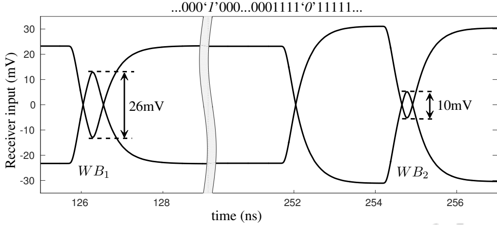
Figure 2.8: Interconnect response to WC_1 and WC_2 for more than optimum pre-emphasis: WB_2 has minimum eye opening at Receiver input.
