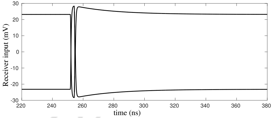
Figure 2.9: Interconnect response to WC_1 and WC_2 for more than optimum pre-emphasis, indicating the long time taken to reach steady state.
