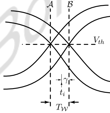
Figure 6.15: Cartoon of an eye diagram with ISI limited to 1 previous bit.
