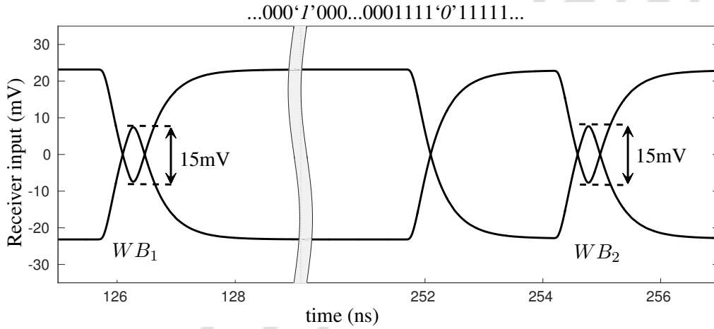
Figure 2.11: Interconnect response to WC_1 and WC_2 for optimum pre-emphasis: WB_1 and WB_2 have equal eye opening.
