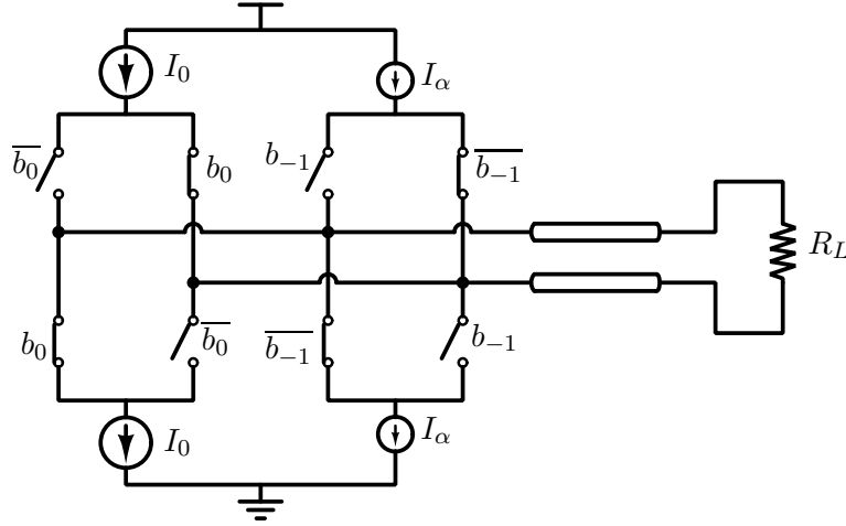
Figure 2.5: A 1 tap FFE transmitter implemented using charge steering current mode transmitter.
