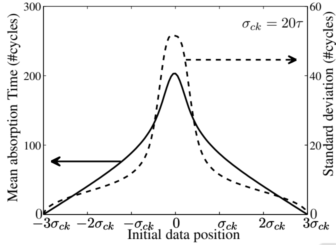
Figure 6.23: Mean absorption time and standard deviation of the absorption time with Gaussian distributed random jitter. The standard deviation of the clock jitter is assumed to be 20\tau (i.e. 0.02\text{UI} ).
