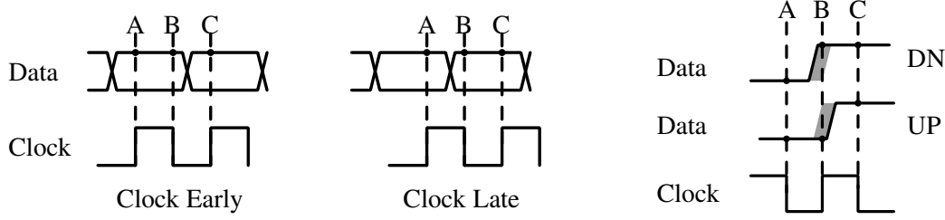
(a) Sampling instants of the phase detector.
