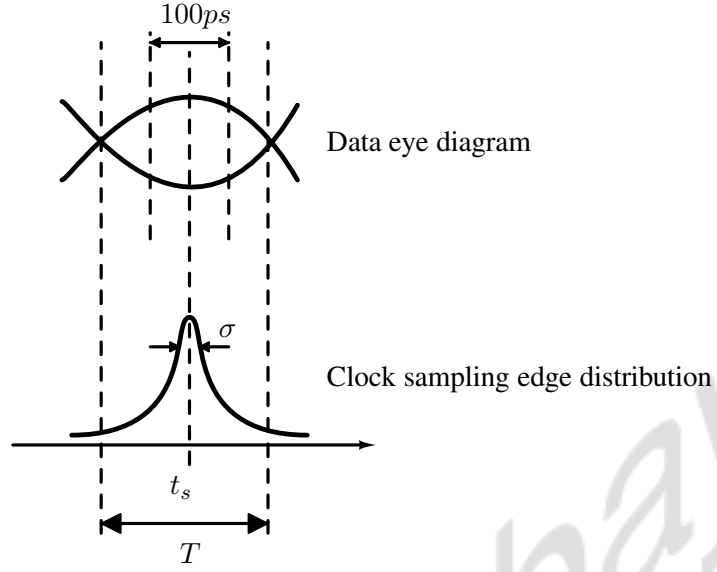
Figure 4.1: Illustration of typical eye diagram at receiver input for low swing interconnects. T is the clock period and \sigma is the standard deviation of the jitter in the clock.
