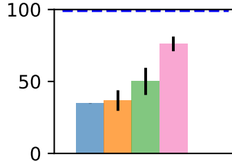
CartPole
