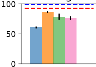
Pong
