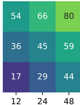
Boxing
