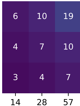
Pong
