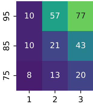
CartPole
