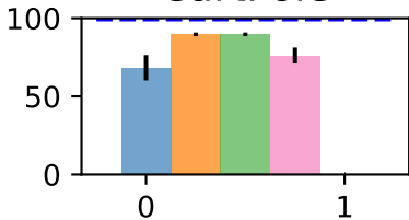
CartPole
