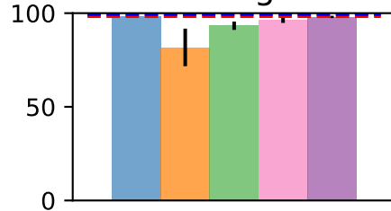
Pong
