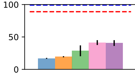
CartPole
