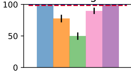
Boxing
