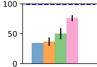
CartPole
