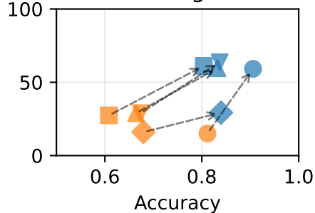
Pong
