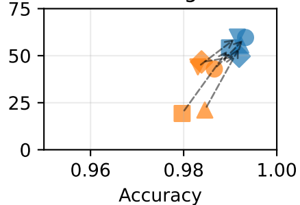
Boxing
