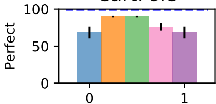
CartPole
