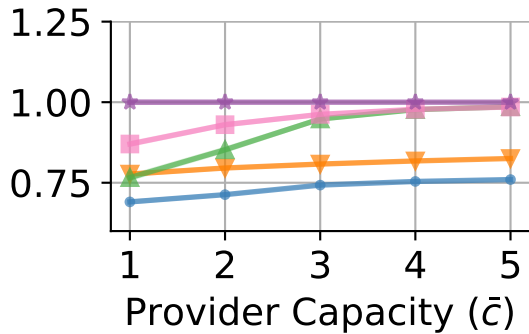
Normalized Utility
