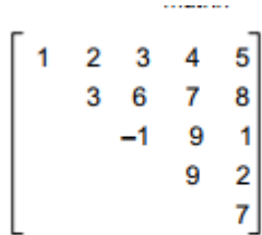
Figure 3.35 Upper-triangular matrix
