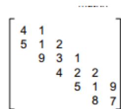
Figure 3.36 Tri-diagonal matrix
