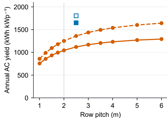
Yield per installed capacity
