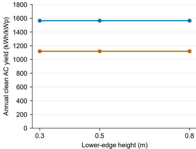
Height sensitivity of infinite-sheds model
