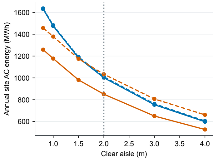
Matched aisle comparison
