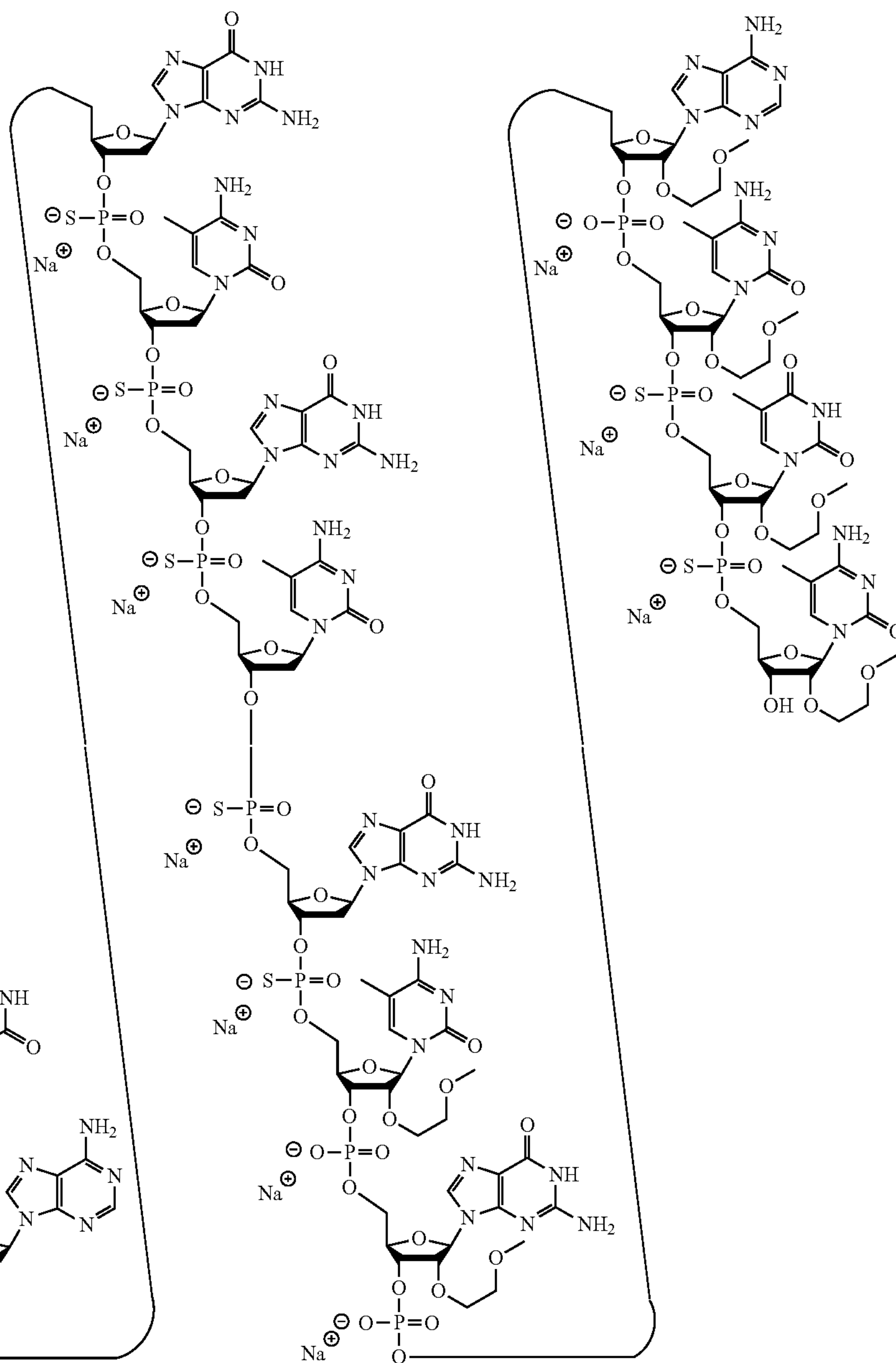
Structure 2. The Sodium Salt of ISIS 801287
