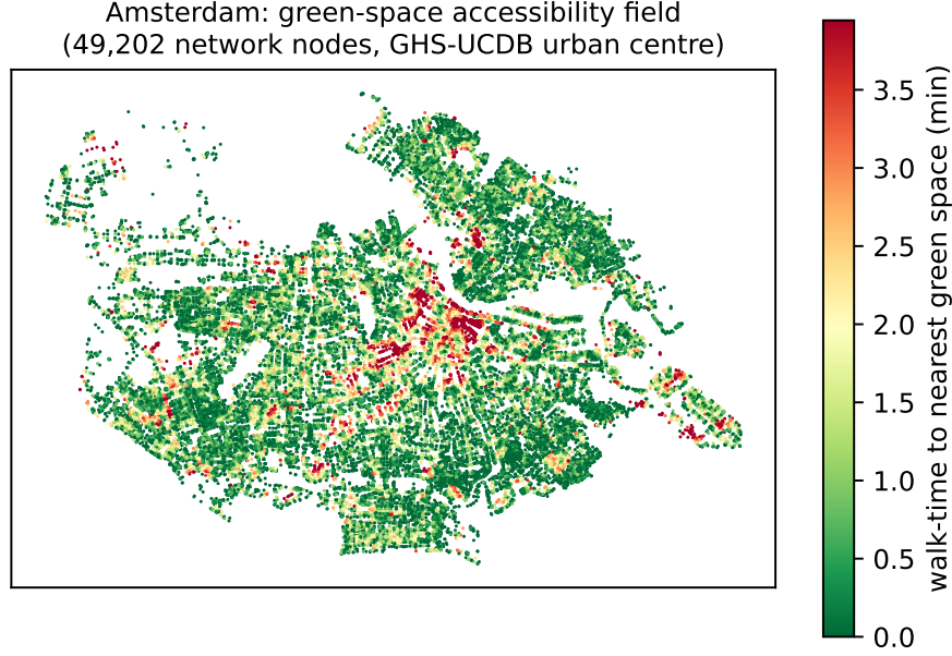
Figure 1: Green-space accessibility field for Amsterdam: each of the 49,202 pedestrian-network nodes inside the GHS-UCDB urban centre, coloured by network walking time to the nearest green space. Green marks well-served locations, red the access-poor pockets whose merging structure the resilience metric tracks.
