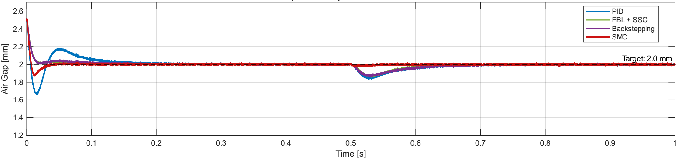
Air Gap Time Response — All Controllers
