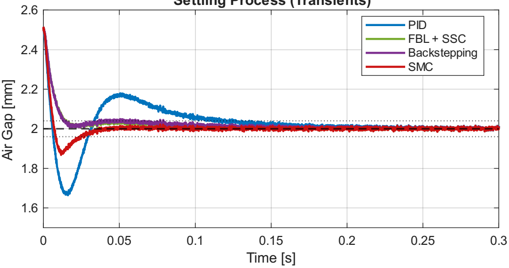
Settling Process (Transients)
