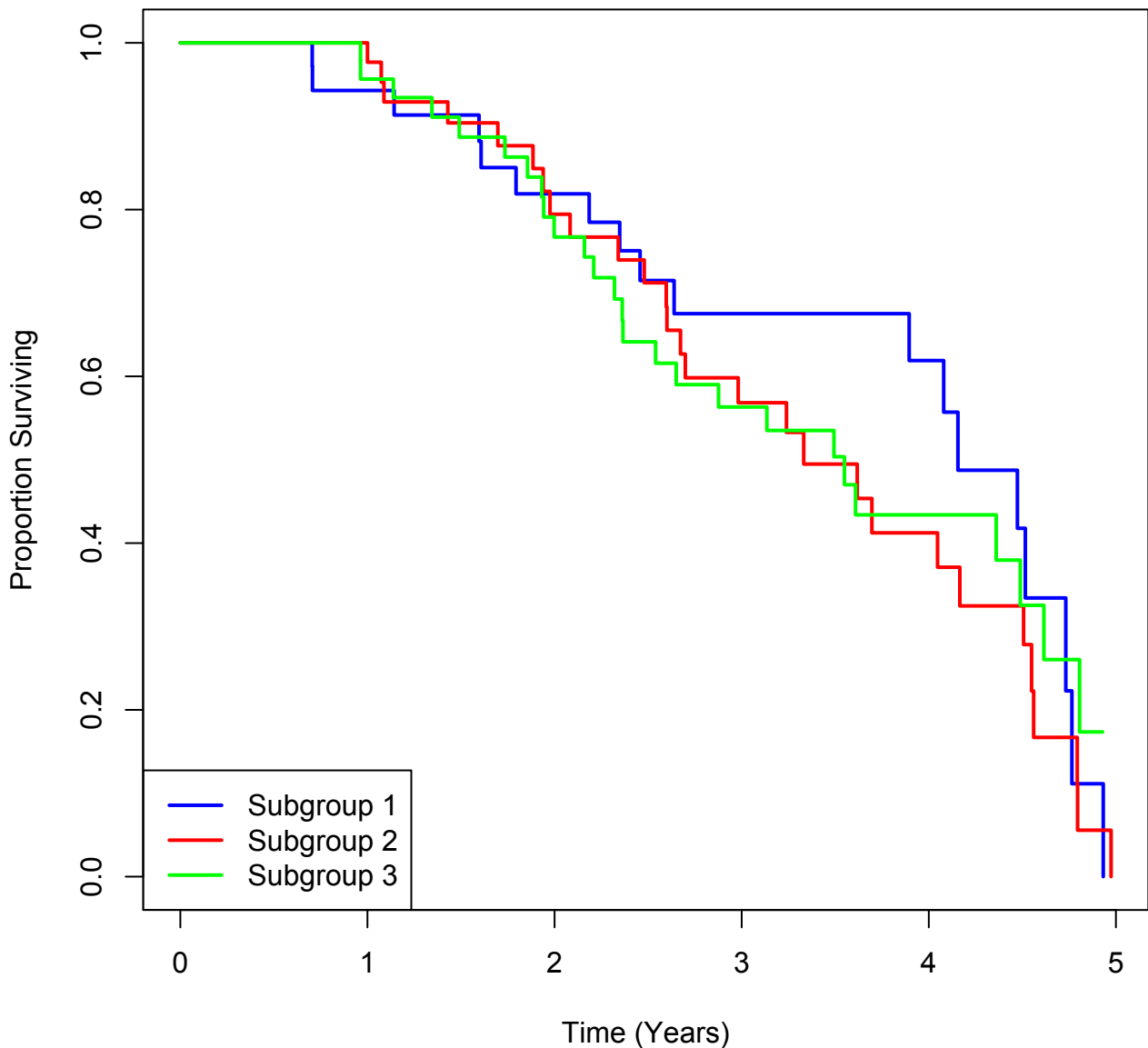
Overall Survival of Prognostic Subgroups
