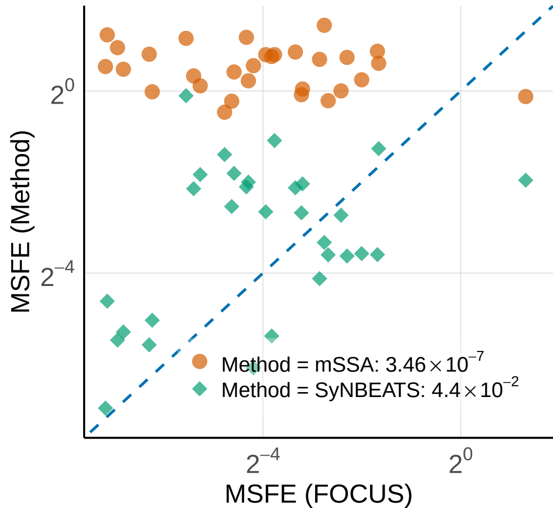
DGP-2, h = 2 ( T = 32 )
