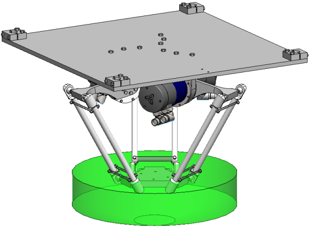
Delta Robot
