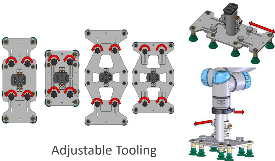
SolidWorks Assembly
