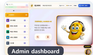
Admin dashboard
