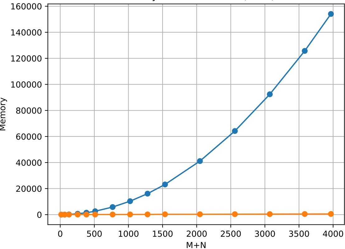
Memory vs Problem Size (M+N)
