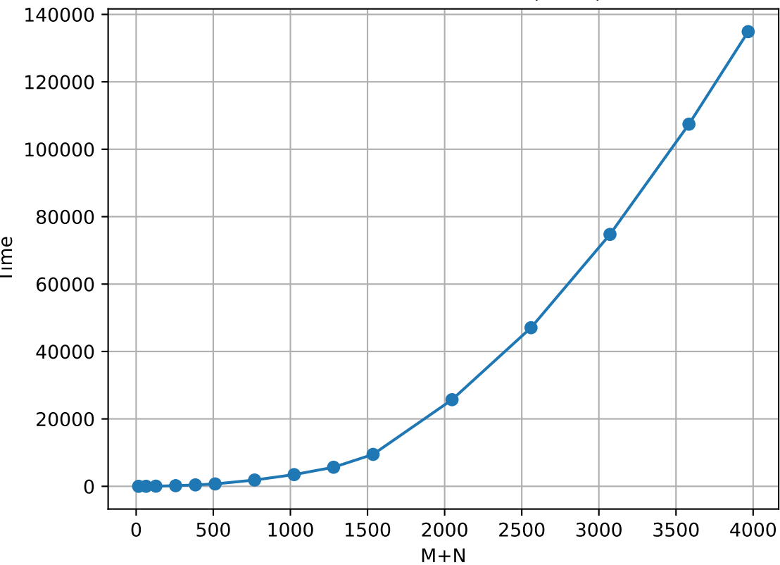
Time vs Problem Size (M+N)
