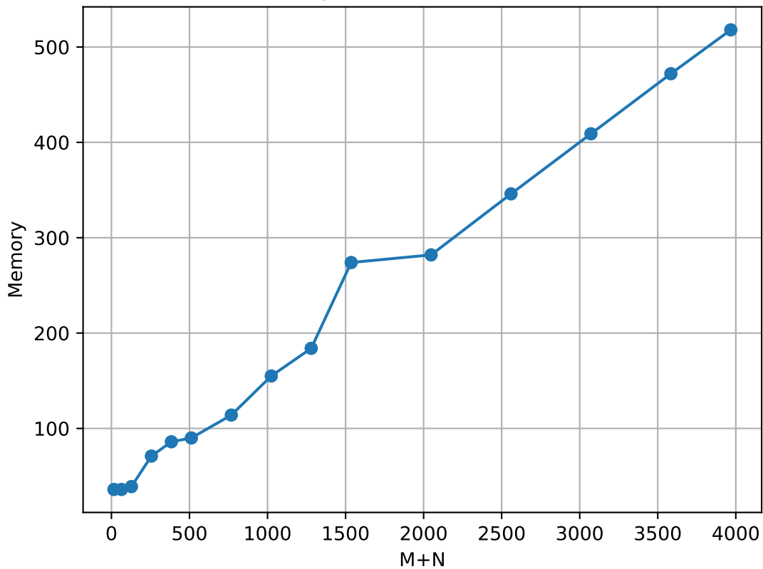
Memory vs Problem Size (M+N)
