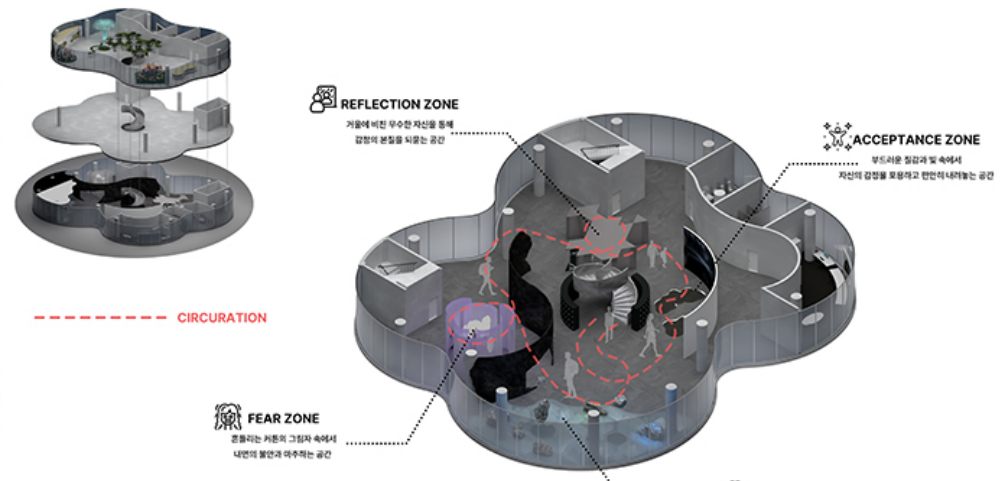
ISOMETRIC_B1F
