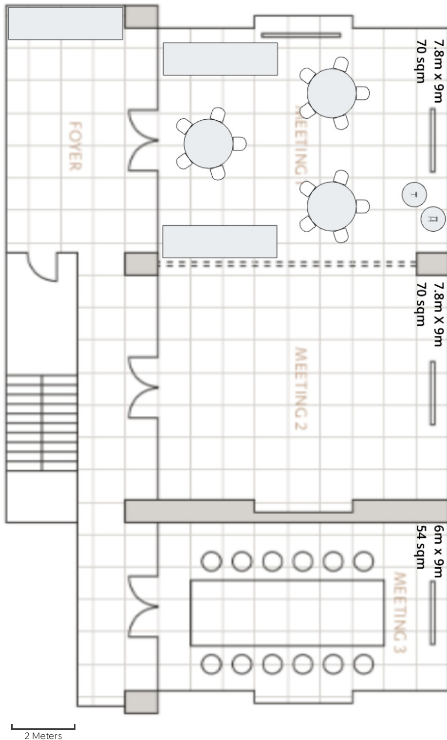
Figure 4: Here is an example layout for a 70sqm space at the Shilla Monogram hotel in Da Nang, Vietnam. Notice that 70 square meters is just barely enough space for 3 tables of 5 students each. This only works because one of the whiteboards has been placed in the foyer. Otherwise only 2 tables of 5 students would fit.
