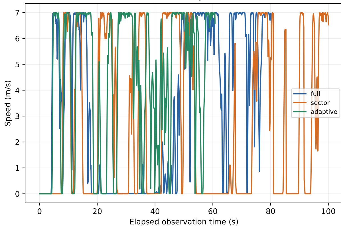
Measured speed
