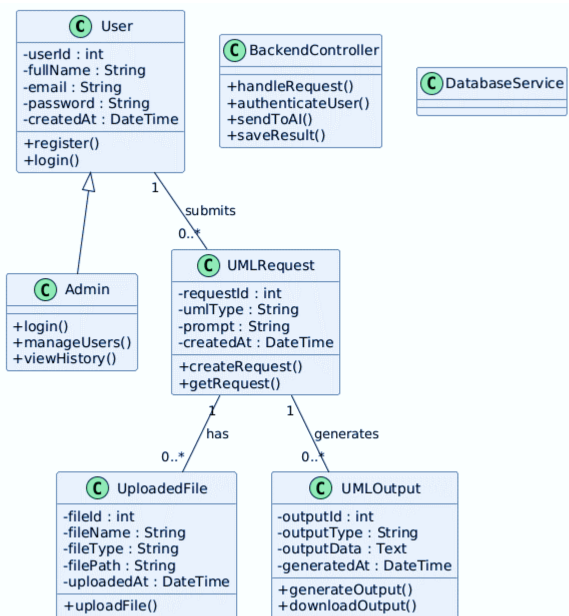
Figure 9: Class Diagram
