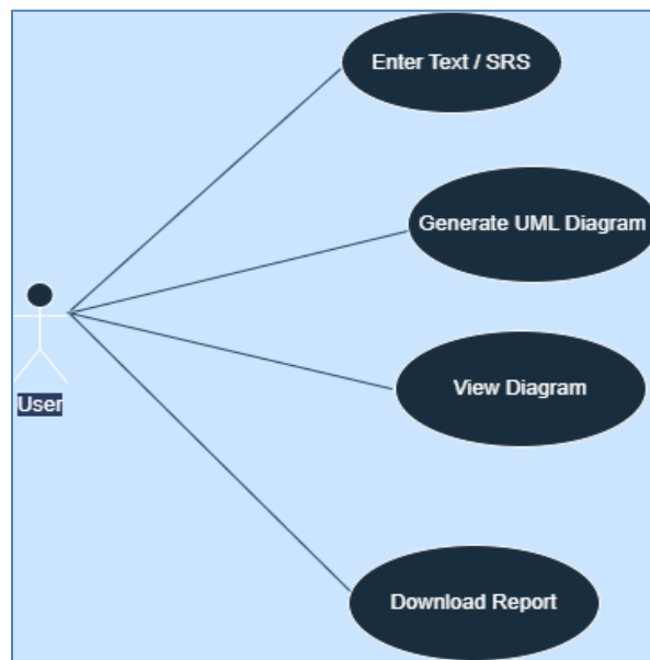
Figure 4: UML Generation
