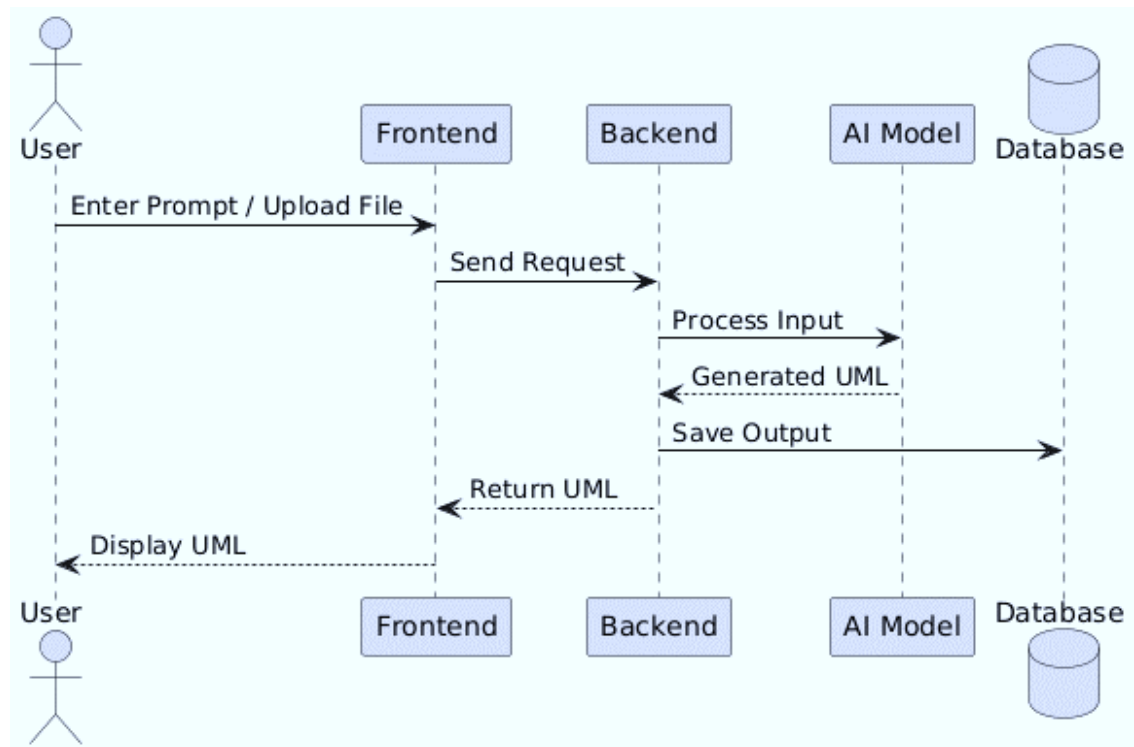
Figure 7: Sequence Diagram
