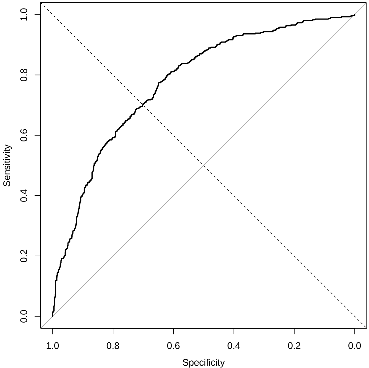
ROC Curve | AUC = 0.776
