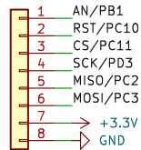
J109 Conn_01x08
