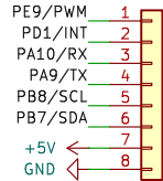
J106 Conn_01x08
