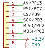
J105 Conn_01x08
