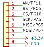
J101 Conn_01x08
