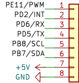
J108 Conn_01x08
