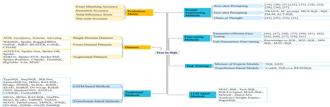
Fig. 2. The overview of the text-to-SQL metrics, datasets, and methods.
