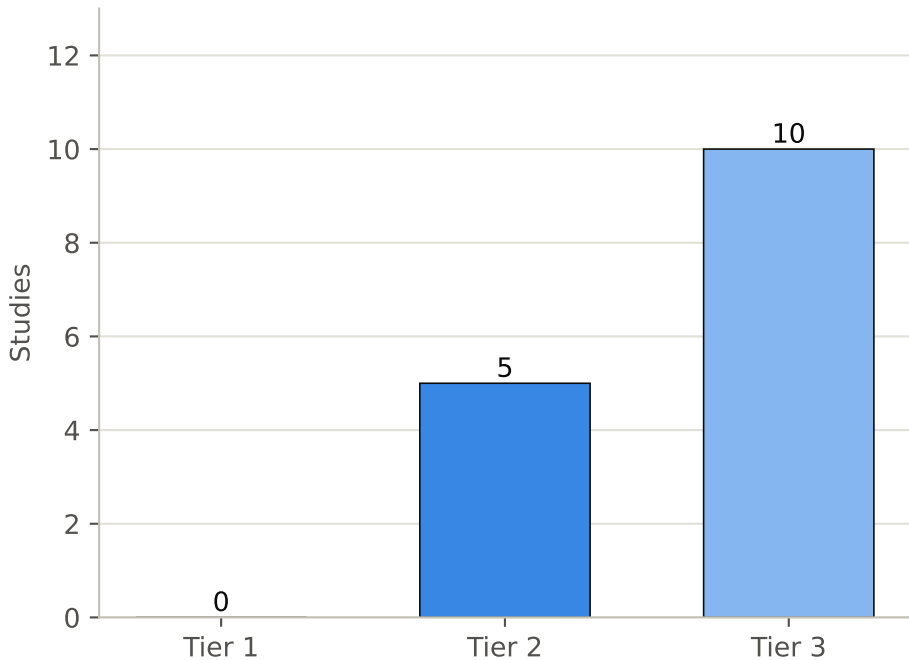
Venue-tier distribution (n = 15)
