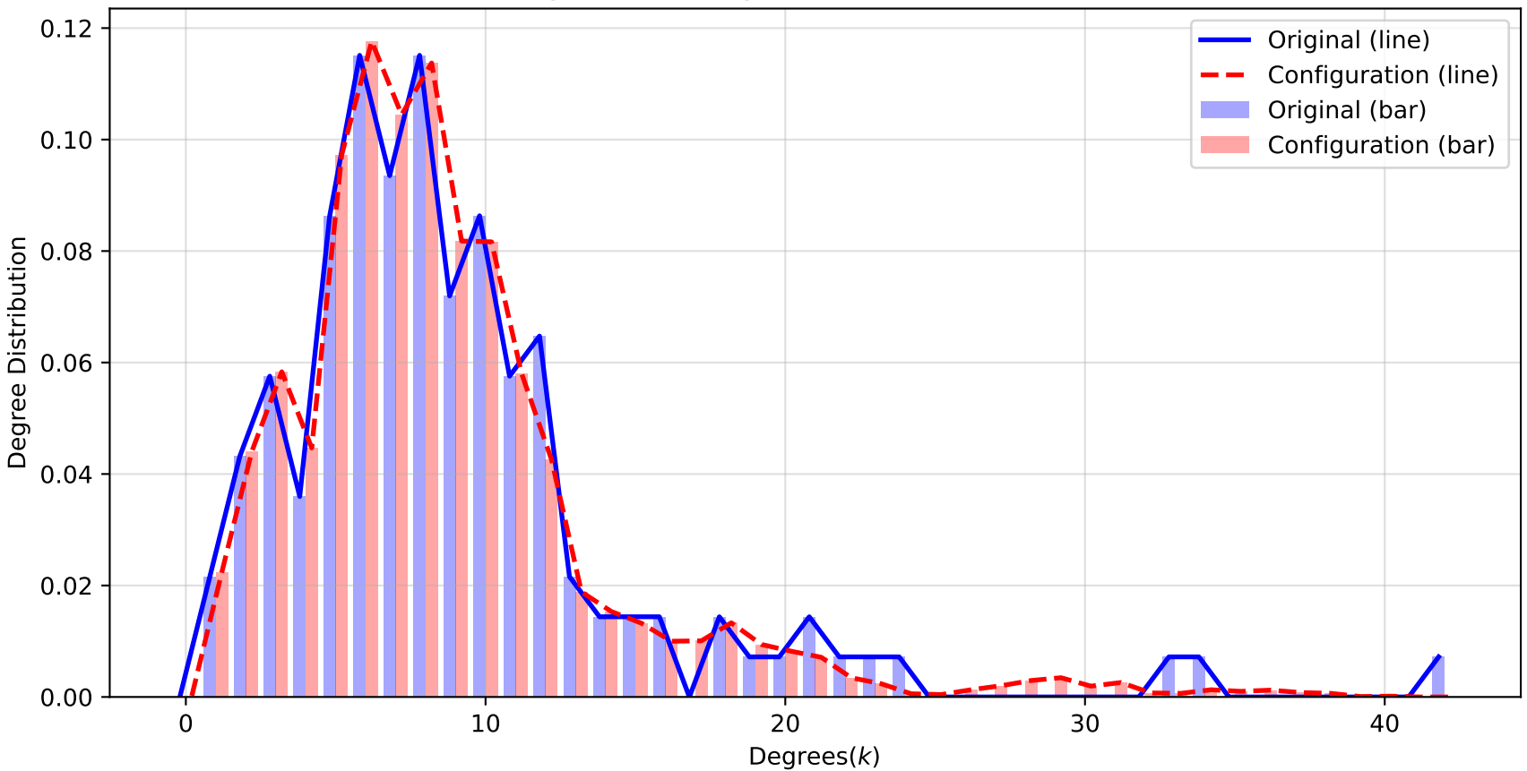
Original vs Configuration (ensemble = 100)
