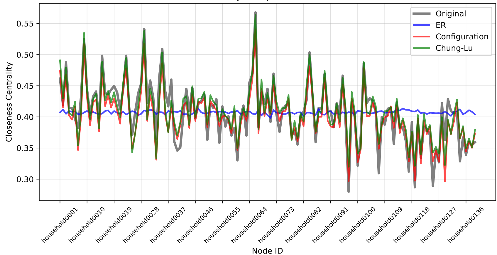
Closeness Centrality Comparison (ensemble = 100)
