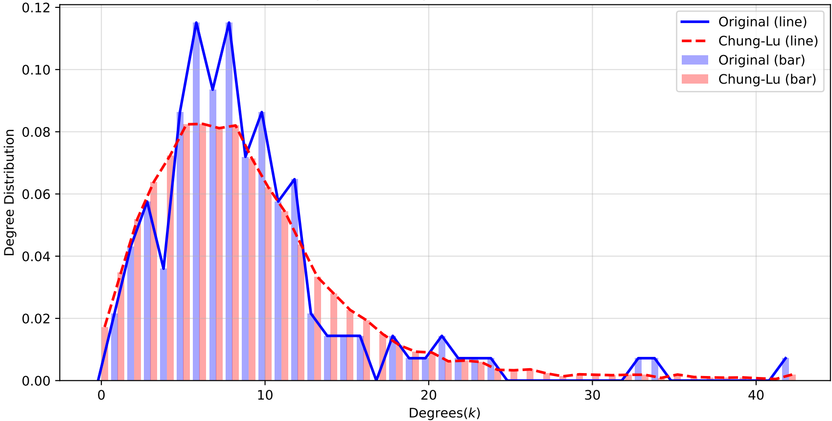
Original vs Chung-Lu (ensemble = 100)
