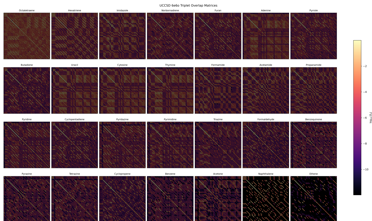
Figure S7: Full 28-molecule triplet overlap heatmaps comparing statevector and shot-based results.
