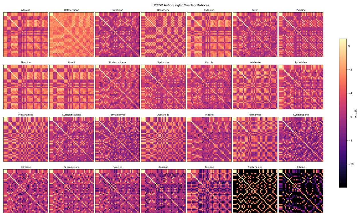
Figure S6: Full 28-molecule singlet overlap heatmaps comparing statevector and shot-based results.
