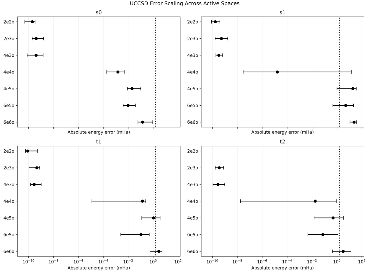
Figure 2: Dependence of UCCSD QSE energy errors on active-space size. Results are shown for the lowest singlet and triplet states across the 2e20 , 2e30 , 4e30 , 4e40 , 4e50 , 6e50 , and 6e60 active spaces. Markers and horizontal error bars summarize the central error and spread across the molecular benchmark, while the dotted line denotes chemical accuracy.
